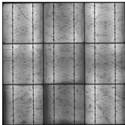
Figure 9. EL image of a mini-module after 1000 h of damp-heat.
