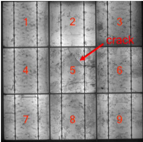
(a) EL image of the PV mini-module after production.
