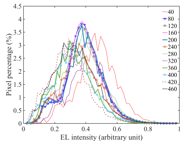
Figure 6. Histograms of the EL intensities after 40, 80, 120, 160, 200, 240, 280, 320, 360, 400, 420 and 460 cycles for the whole mini-module.
