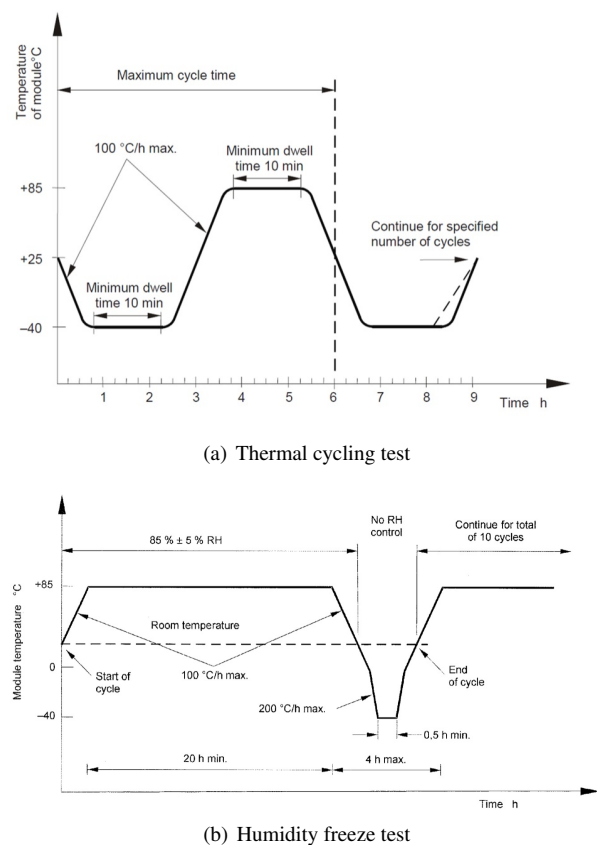
Figure 1. Accelerated ageing tests prescribed by IEC standards 20 .
