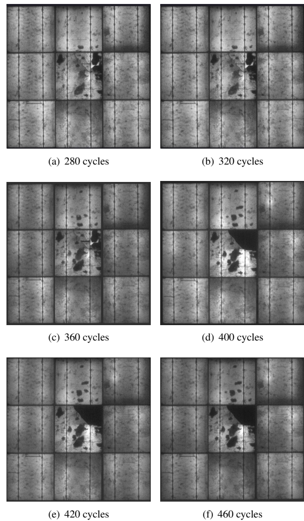
Figure 5. Electroluminescence images during accelerating ageing after: (a) 280 cycles; (b) 320 cycles; (c) 360 cycles; (d) 400 cycles; (e) 420 cycles; (f) 460 cycles.
