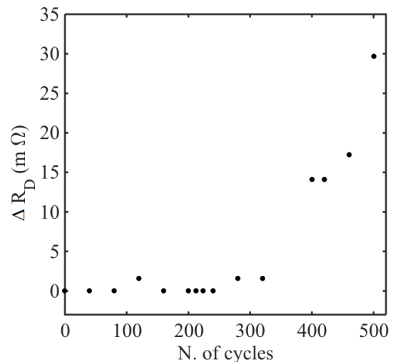
Figure 8. Evolution of the degradation of the electric resistance over time.
