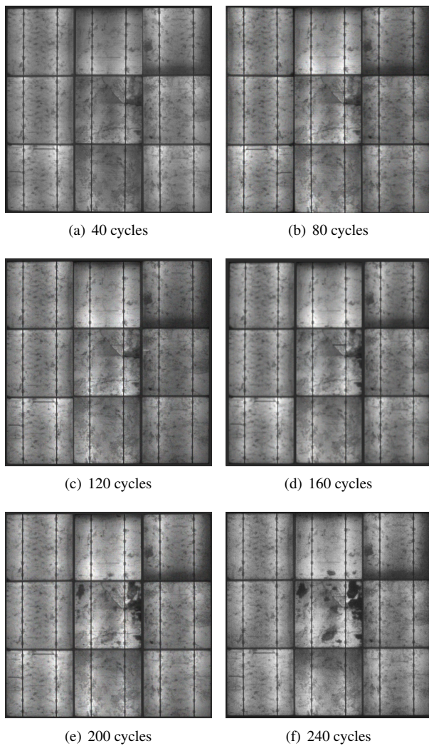
Figure 4. Electroluminescence images during accelerating ageing after: (a) 40 cycles; (b) 80 cycles; (c) 120 cycles; (d) 160 cycles; (e) 200 cycles; (f) 240 cycles.
