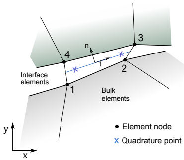
Fig. 6: Sketch of the interface finite element topology.
