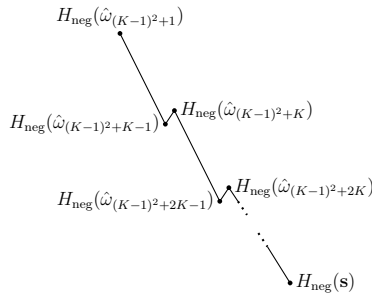
Figure 5: Qualitative illustration of the energy of the configurations belonging to \hat{\omega}^{(2)} .
