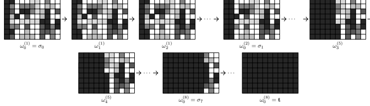
Figure 14: Illustration of some particular configurations belonging to the path \omega : \sigma \rightarrow \mathbf{t} of Proposition 4.4. We color black those vertices whose spin is t .
