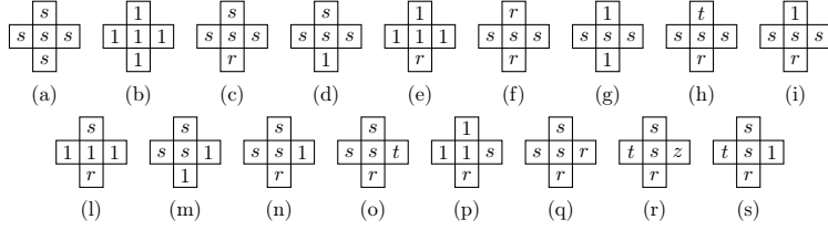
Figure 6: Stable tiles centered in any v \in V for a q -Potts configuration \sigma on \Lambda for any r, s, t, z \in S \setminus \{1\} different from each other. The tiles are depicted up to a rotation of \alpha \frac{\pi}{2} , \alpha \in \mathbb{Z} .
