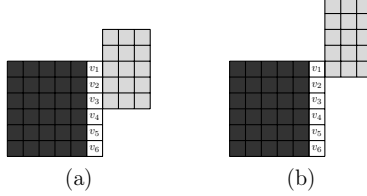
Figure 12: Examples of interacting rectangles in \tilde{\eta} when \ell^* = 5 . We color gray the r -rectangle \hat{R} and black the s -rectangle.
