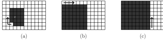
Figure 4: (a) First steps of path \hat{\omega}^{(2)} on a 10 \times 12 grid \Lambda starting from the vertex v = (3, 3) . We color white the vertices with spin 1, black those with spin s . The arrow indicates the order in which the spins are flipped from 1 to s . (b) Illustration of \hat{\omega}_{(K-1)^2} . (c) Illustration of \hat{\omega}_{(K-1)^2+K-1} .
