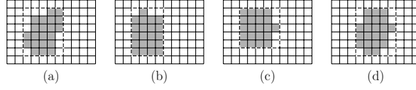
Figure 16: Examples of \sigma \in \tilde{\mathcal{D}}_{\text{neg}}^t in (a) and of \sigma \in \hat{\mathcal{D}}_{\text{neg}}^t in (b) and (c) when \ell^* = 5 . We associate the color gray to the spin t , the color white to the spin 1. The dashed rectangle represents the smallest surrounding rectangle of C^t(\sigma) . Figure (d) is an example of configuration that does not belong to \hat{\mathcal{D}}_{\text{neg}}^t .
