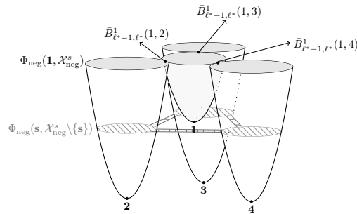
Figure 1: Schematic picture of the energy landscape below \Phi_{\text{neg}}(\mathbf{1}, \mathcal{X}_{\text{neg}}^s) of the 4-state Potts model with negative external magnetic field with S = \{1, 2, 3, 4\} , \mathcal{X}_{\text{neg}}^s = \{\mathbf{2}, \mathbf{3}, \mathbf{4}\} . We have not represented the cycles (valleys) that contain configurations with stability level smaller than or equal to 2 (see Proposition 3.2).
