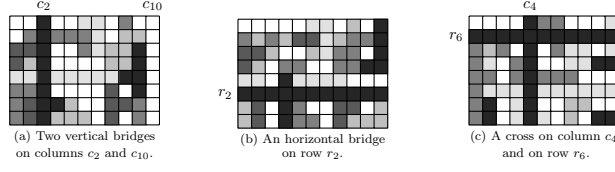
Figure 3: Example of configurations on a 8 \times 11 grid graph displaying a vertical s -bridge (a), a horizontal s -bridge (b) and a s -cross (c). We color black the spins s .
