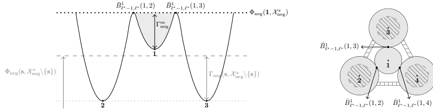
Figure 2: On the left, we give a side view (vertical section) of the energy landscape depicted in Figure 1. We colour light gray the initial cycle \mathcal{C}_{\mathcal{X}_{\text{neg}}^s}^{\mathbf{1}}(\Gamma_{\text{neg}}^m) . On the right, viewpoint from above of the energy landscape depicted in Figure 1 cut to the energy level \Phi_{\text{neg}}(\mathbf{1}, \mathbf{s}) , for some \mathbf{s} \in \mathcal{X}_{\text{neg}}^s . The dashed part denotes the energy landscape whose energy value is smaller than \Phi_{\text{neg}}(\mathbf{1}, \mathbf{s}) . The cycles whose bottom is a stable state are deeper than the cycle \mathcal{C}_{\mathcal{X}_{\text{neg}}^s}^{\mathbf{1}}(\Gamma_{\text{neg}}^m) of the metastable state, hence we depict them with circles whose diameter is larger than the one related to the metastable state \mathbf{1} .
