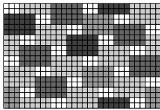
Figure 13: Local minimum on a 30 \times 20 grid graph in which there are not any s -rectangle with at least a side neither completely adjacent to an r -cluster nor completely surrounded by spins 1.
