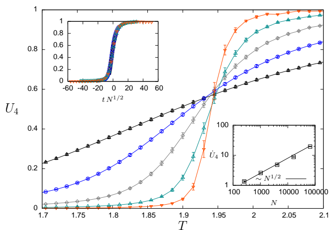
FIG. 10: Binder cumulant versus temperature for \rho = 2.333 in the mean-field regime. The upper inset shows the scaling (19) with \bar{\nu} = 2.00(3) and the lower inset is the calculation of \bar{\nu} with the relation (30).
