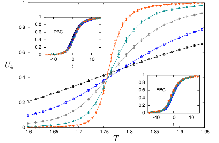
FIG. 14: Binder cumulant versus temperature for \rho = 10/3 in the non-mean-field regime. The upper inset shows the scaling as in figure 10 with \bar{\nu} = 2.19(2) , while the lower inset shows the scaling into the \rho = 10/3 system with FBC and with \bar{\nu} = 2.24(4) .
