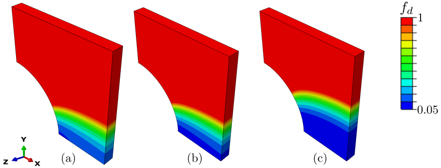
Fig. 7: Isocontour plots for the damage function f_d of a plate with a hole plotting the crack pattern for several displacements: (a) u_z = 7.32 mm, (b) u_z = 8.42 mm and (c) u_z = 19.10 mm. Employed non-local damage parameters encompass: \eta_d = 1 MPa ^{-1} , \kappa_d = 1 MPa and c_d = 500 MPa ^{-1} mm ^2
