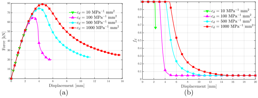
Fig. 11: (a) Reaction force-displacement and (b) minimum value of f_d curves for the plate with a hole problem run with a standard spatial CDM approach for different cases of c_d = \{10, 100, 500, 1000\} \text{ MPa}^{-1} \text{ mm}^2 .
