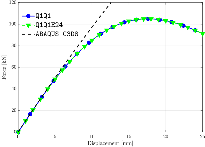
Fig. 6: Reaction force-displacement curves for the compressible plate with a hole for the validation probes conducted with a standard CDM (Q1Q1) and CDM + EAS (Q1Q1E24), respectively, compared with ABAQUS C3D8 elements. Employed non-local damage parameters encompass: \eta_d = 0.1 \text{ MPa}^{-1} , \kappa_d = 0 \text{ MPa} and c_d = 1000 \text{ MPa}^{-1}\text{mm}^2 .
