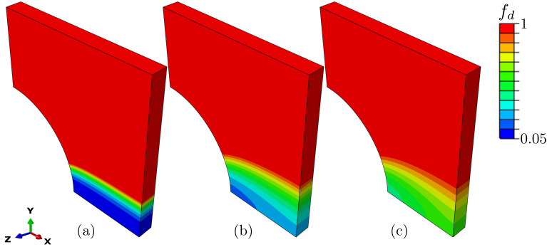
Fig. 10: Isocontour plots for the damage function f_d for plates with a hole at u_z = 6.5 mm. In here: (a) c_d = 100 \text{ MPa}^{-1}\text{mm}^2 , (b) c_d = 500 \text{ MPa}^{-1}\text{mm}^2 and (c) c_d = 1000 \text{ MPa}^{-1}\text{mm}^2 .
