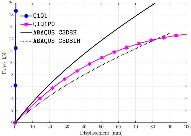
Fig. 21: Load-displacement curves for the incompressible cylindrical shell test conducted for Q1Q1 and Q1Q1P0 formulations compared with the ABAQUS hybrid theoretical curves with (C3D8H) and without considering incompatible modes (C3D8IH). The employed saturation parameter has been \eta_d = 0.1 \text{ MPa}^{-1} .
