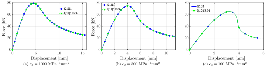
Fig. 9: Reaction force-displacement curves for the compressible plate with a hole problem comparing standard CDM (Q1Q1) and CDM + EAS (Q1Q1E24) formulations varying c_d .
