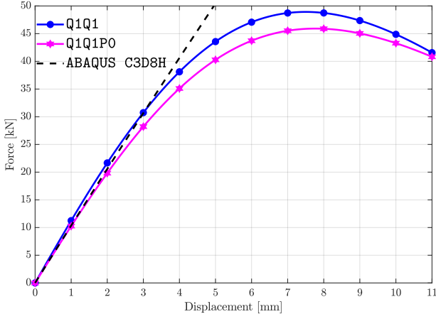
Fig. 12: Reaction force-displacement curves for the nearly incompressible plate with a hole for the validation probes conducted with a standard (Q1Q1) and the mixed u-p-J CDM formulations (Q1Q1P0), respectively, compared with ABAQUS C3D8H elements. Employed non-local damage parameters encompass: \eta_d = 0.5 \text{ MPa}^{-1} , \kappa_d = 0 \text{ MPa} and c_d = 1000 \text{ MPa}^{-1}\text{mm}^2 .
