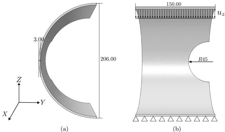
Fig. 15: Geometry with boundary conditions and dimensions in mm with (a) profile and (b) frontal view.
