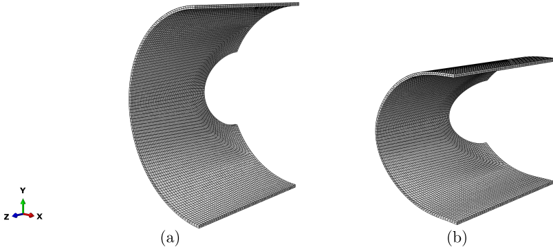
Fig. 16: Cylindrical shell: undeformed and deformed configuration.
