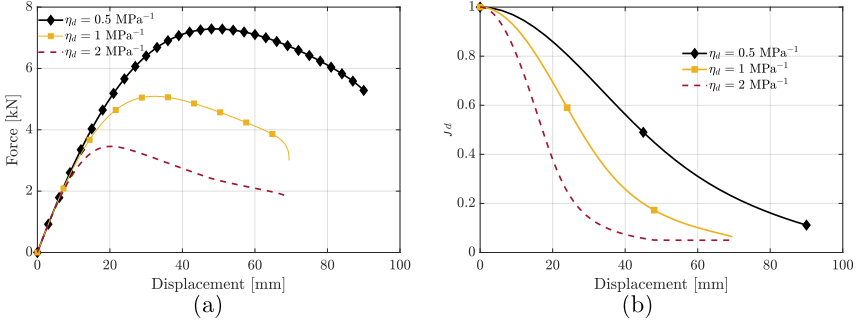
Fig. 22: (a) Reaction force-displacement and (b) minimum value of f_d -displacement curves for incompressible cylindrical shells under bending loads conducted with a mixed u-p-J CDM (Q1Q1P0) approach for different cases of \eta_d = \{0.5, 1, 2\} \text{ MPa}^{-1} .
