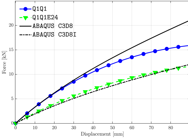
Fig. 17: Load-displacement curves for the cylindrical shell test conducted for Q1Q1 and Q1Q1E24 formulations compared with the ABAQUS theoretical curves with (C3D8I) and without considering incompatible modes (C3D8). The employed saturation parameter has been \eta_d = 0.1 \text{ MPa}^{-1} .
