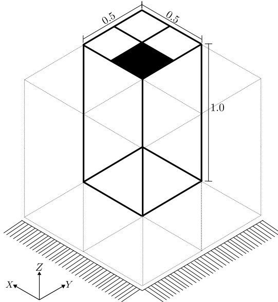
Fig. 1: Scheme for the block under compressive load modelled. The area in bold corresponds with the region where the compressive u_z is applied on. The dimensions are given in mm. Dotted lines correspond to the regions generated by symmetry.
