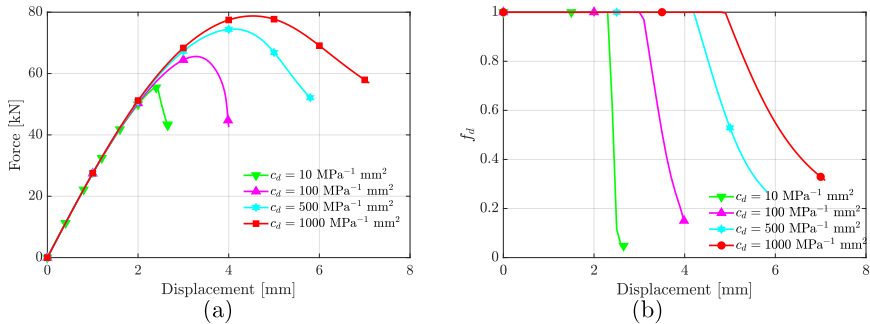
Fig. 14: (a) Reaction force-displacement and (b) minimum value of f_d -displacement curves for the nearly incompressible plate with a hole problem run with a mixed u-p-J CDM (Q1Q1P0) approach for different cases of c_d = \{10, 100, 500, 1000\} \text{MPa}^{-1} \text{mm}^2 .
