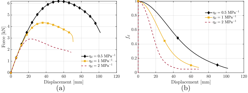
Fig. 20: (a) Reaction force-displacement and (b) minimum value of f_d -displacement curves for compressible cylindrical shells under bending loads conducted with a CDM + EAS (Q1Q1E24) approach for different cases of \eta_d = \{0.5, 1, 2\} \text{ MPa}^{-1} .
