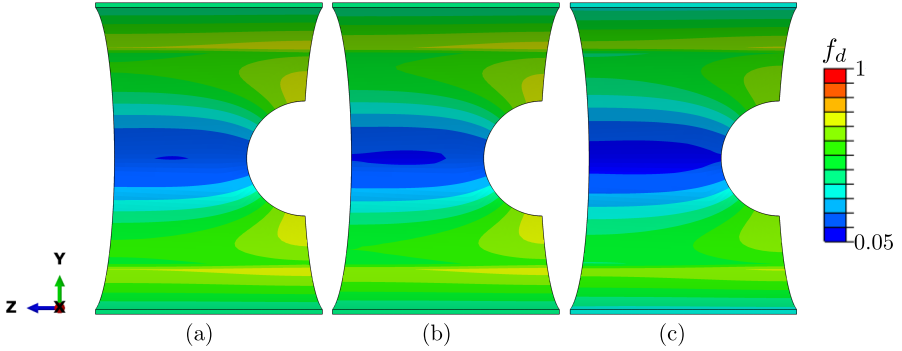
Fig. 18: Isocontour plots for the evolution of the damage function f_d for a compressible cylindrical shell under bending load. It has been employed a saturation parameter for damage of \eta_d = 0.5 \text{ MPa}^{-1} for the Q1Q1E24 formulation.
