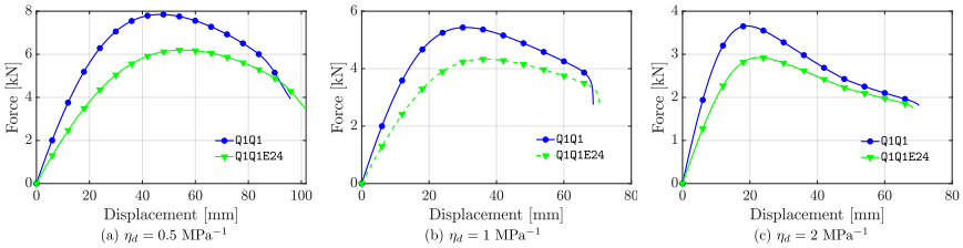
Fig. 19: Load-displacement curves for compressible cylindrical shells under bending load conducted with formulations for standard CDM (Q1Q1) and the CDM + EAS (Q1Q1E24) approaches, respectively with different \eta_d .
