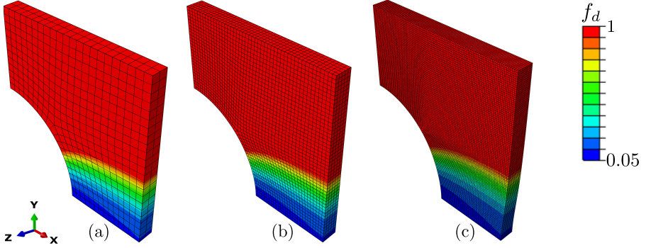
Fig. 8: Isocontour plots for the damage function f_d comparing a (a) coarse, (b) medium-sized, and (c) fine discretisation of a plate with a hole with a fixed displacement of u_z = 8 mm. The obtained results are similar for Q1Q1 and Q1Q1E24 formulations.
