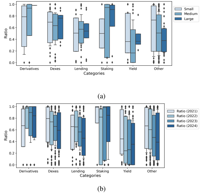
Fig. 9: Ratio of Total Value Redeemable over Total Value Locked. Protocols are grouped by category and further divided by size (a) and time (b). The y-axis indicates the ratio R between TVR and TVL. DEXs and Lending protocols rely more on non-redeemable tokens in 2024 w.r.t. earlier years.
