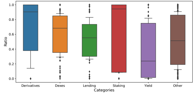
Fig. 8: Ratio R for different protocol categories. We compute R = TVR_a/TVL as the ratio between the value of assets used to measure TVR and the value of TVL, and compare it across protocol categories. Derivatives and staking protocols have the highest R values.
