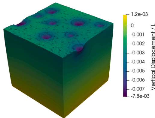
Fig. 12. Deformed configuration of the sample (the deformation is magnified 10× for visualization purposes) for a vertical displacement of 0.25h_{rms} applied to the PS-LDPE sample which is pushed against the rough surface.
