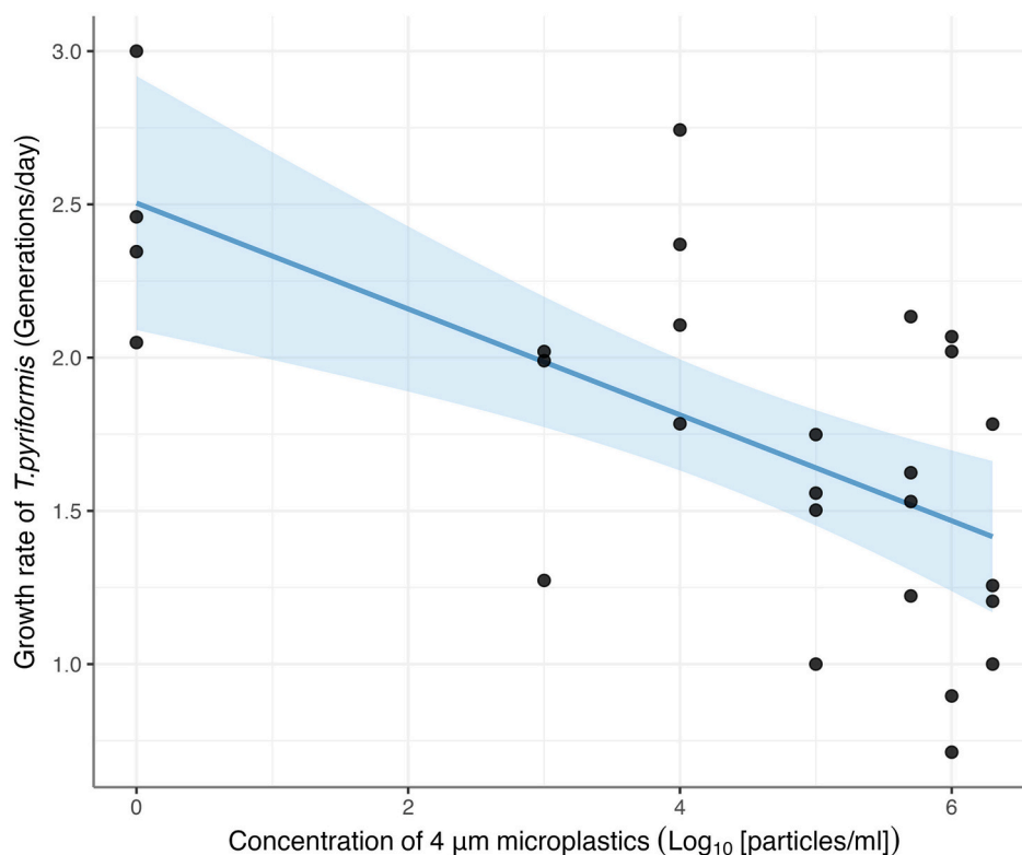
Fig. 3. Growth rate of Tetrahymena pyriformis as a function of microplastic particle concentration. The regression fit is shown including the 95 % confidence interval. T. pyriformis exposed to 10 \mu\text{m} particles (too large to be ingested) is used for microplastic concentration = 0. Microplastic concentrations are \log_{10} + 1 transformed.
