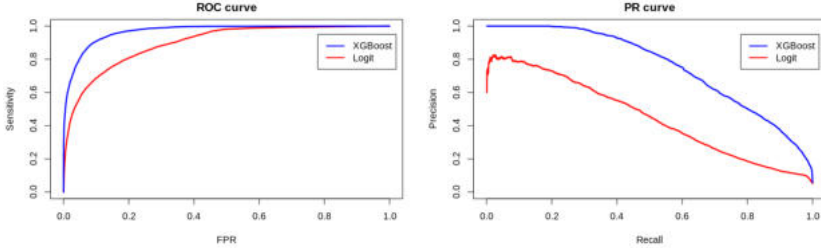
Figure 4: Goodness-of-fit scores
