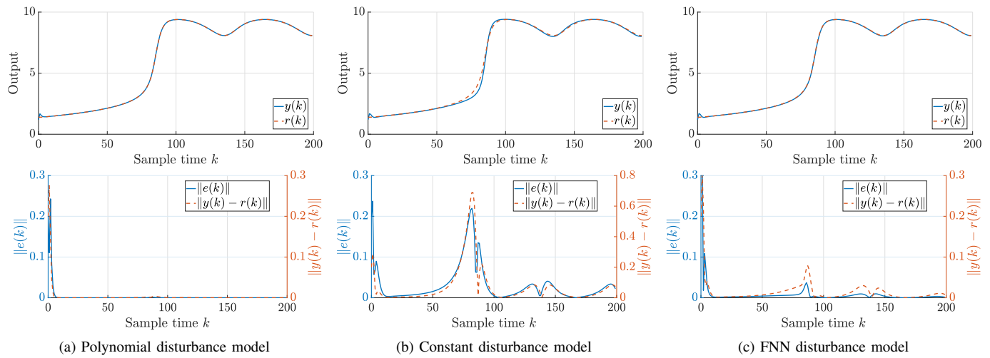
Fig. 4: CSTR plant. Closed-loop tracking of a generic reference trajectory using different disturbance models.
