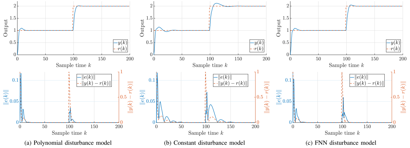
Fig. 2: Van der Pol plant. Closed-loop tracking of a piecewise-constant reference using different disturbance models.
