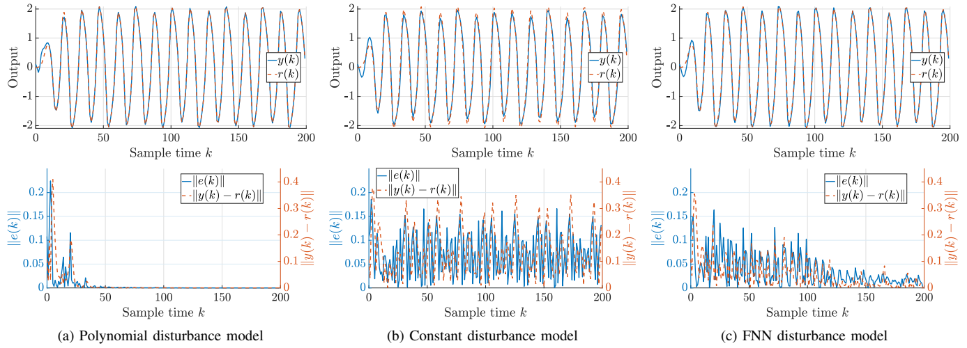
Fig. 3: Van der Pol plant. Closed-loop tracking of a generic reference trajectory using different disturbance models.
