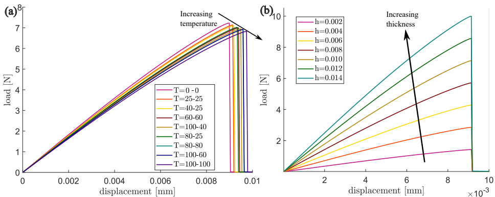
Figure 42: Double-edged notch specimen with (a) reactions for variation of temperatures, (b) reactions for variation of thickness.
