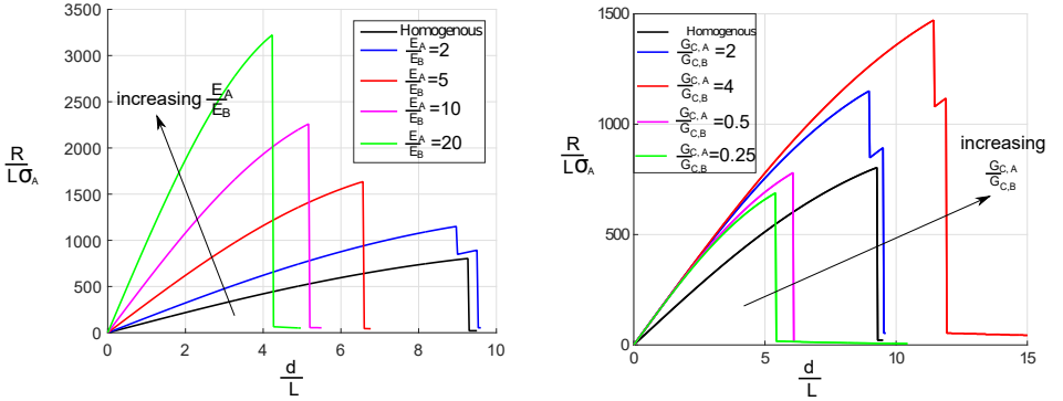
Figure 15: \frac{R}{L\sigma_A} vs \frac{L}{d} ratio for different (left) Young's modulus ratio (right) fracture toughness ratio.
