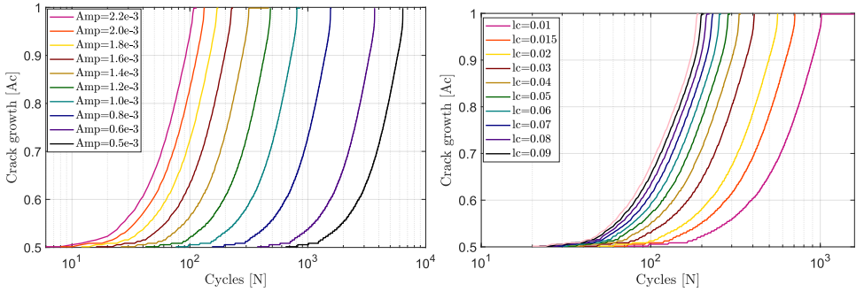
Figure 65: Crack extension vs. number of cycles ( N ) (a) for variation of maximum load amplitude P and, (b) for variation of characteristic length scale l .
