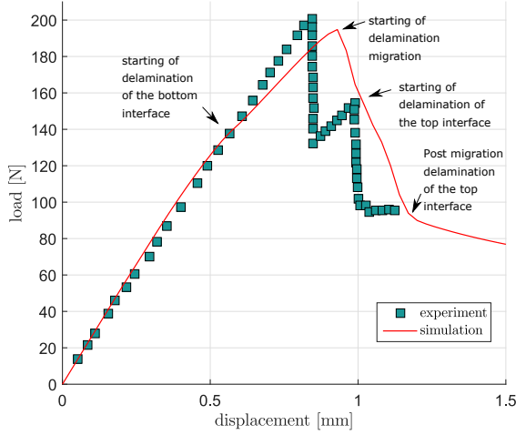
Figure 22: Numerical-experimental correlation corresponding to the load-displacement curve for L = a_0=49 mm.
