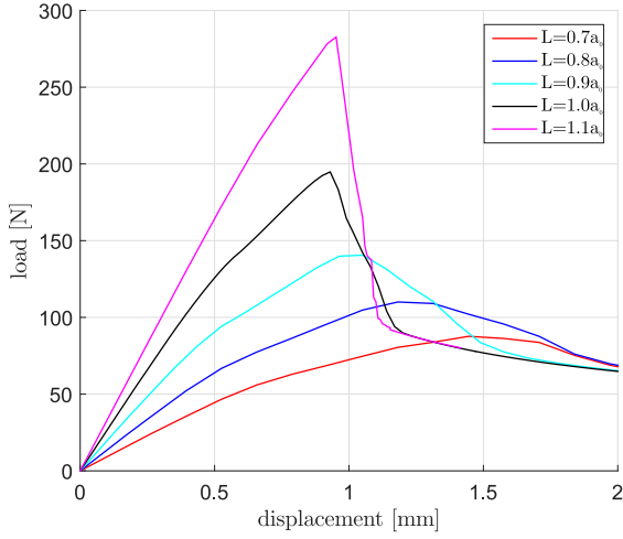
Figure 24: Variation of load across the specimen for a_0 = 49\text{mm} .
