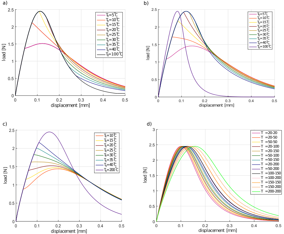
Figure 35: Variation of the reaction forces for different temperature boundary conditions. a) Model-A with T_1 = 50^\circ\text{C} , T_2 = 100^\circ\text{C} . b) Model-B with T_1 = T_2 = 100^\circ\text{C} . c) Model-C with T_1 = T_2 = 200^\circ\text{C} . d) Change of temperature.
