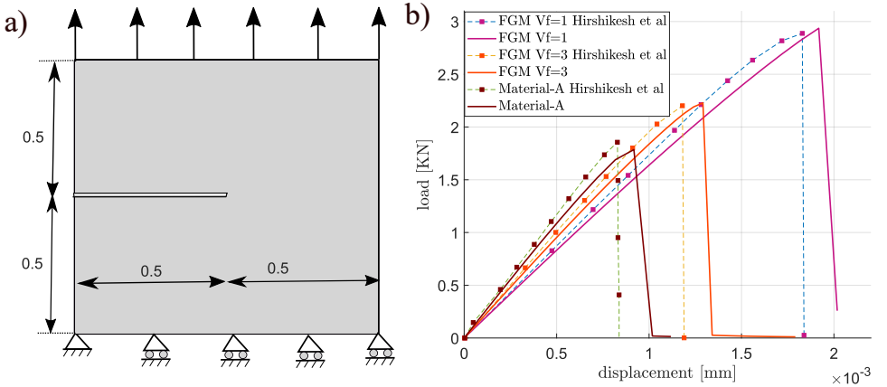
Figure 51: (a) Geometric description of the model, (b) force vs. displacement plots comparison with Hirshikesh et al [90].
