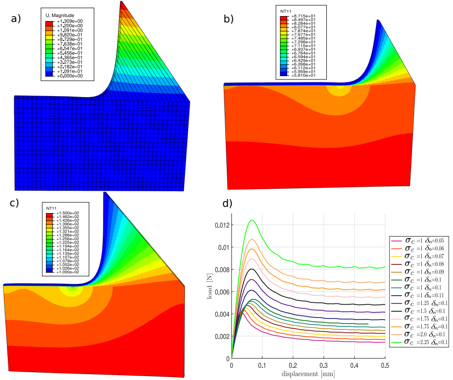
Figure 39: a) Displacement of model-A at time \tau = 1 for load \bar{u} = 1 mm. b) Temperature field for displacement of \bar{u} = 0.07 mm. c) Temperature field for \bar{u} = 1.0 mm. d) Force v/s displacement curves of model-A for the variation of \sigma_c and maximum allowed gaps \delta_n .
