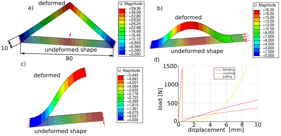
Figure 32: a) Pulling the bar from middle. b) Buckling of the bar. c) Bending thickness of 0.2 mm.
