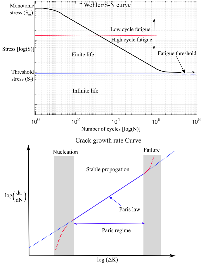
Figure 2: Schematic representation of a) SN curve, and b) Paris law.
