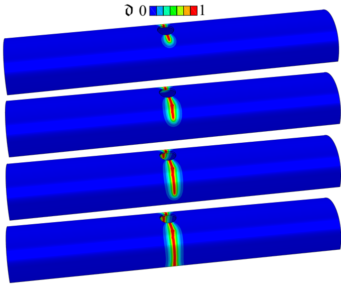
Figure 70: (a) Phase-field crack propagation for cylindrical shell.
