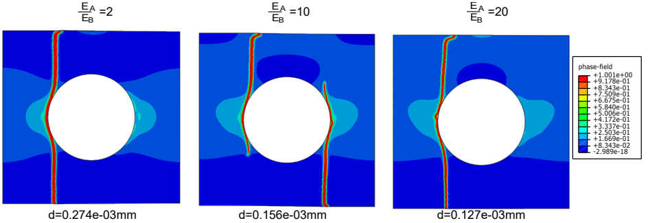
Figure 17: Crack propagation in single fiber reinforced composite.
