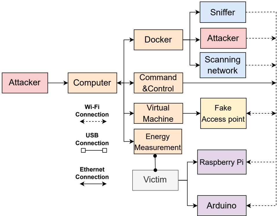
Figure 19. Testing Environment.
