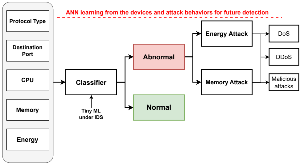
Figure 54. Detection Model.
