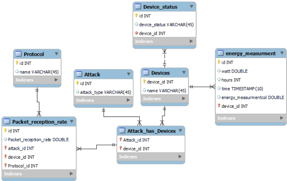
Figure 57. Chapter 4 Database Schema.
