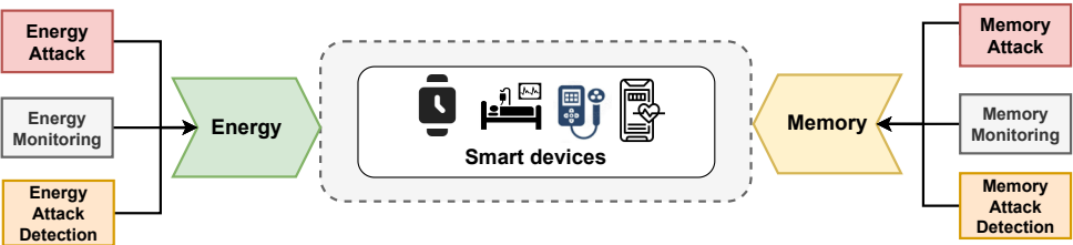
Figure 52. Thesis Conclusions.
