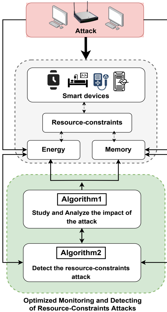
Figure 5. Main Contributions.
