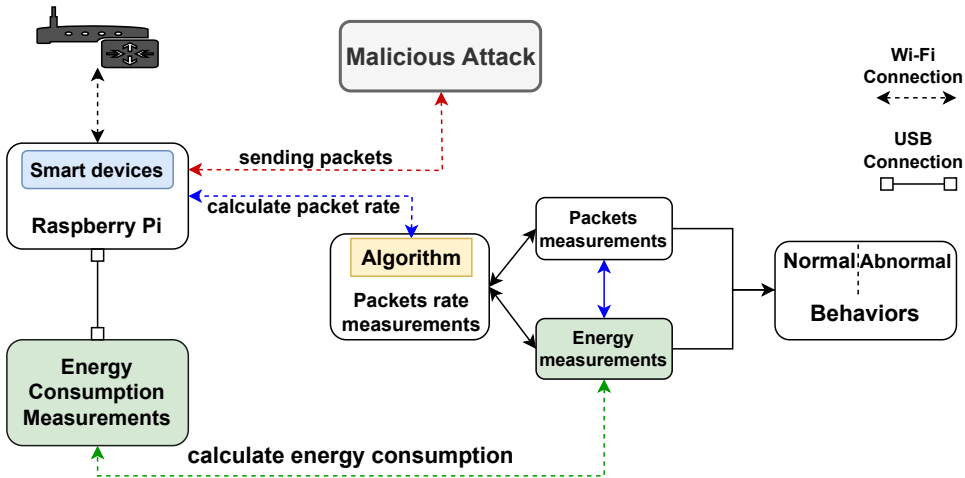
Figure 33. Testing Environment.
