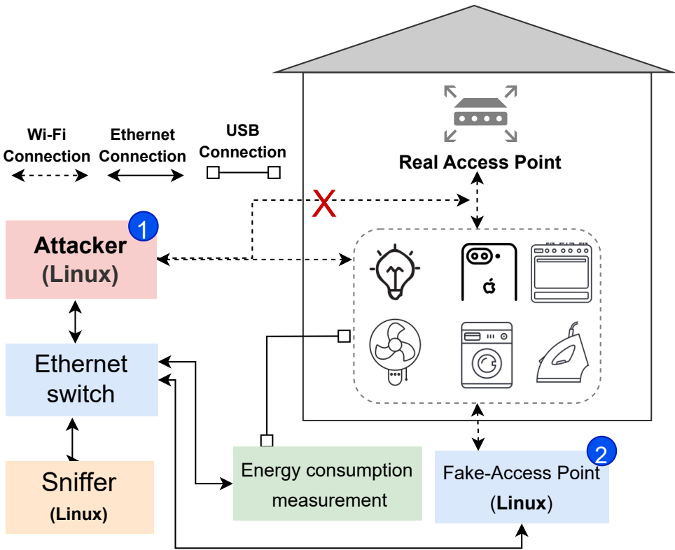
Figure 20. Attacking Scenarios.
