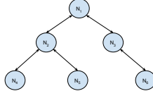
Figure 80: Tree topology.
