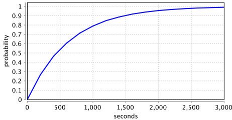
Figure 82: Probability of mining a block.
