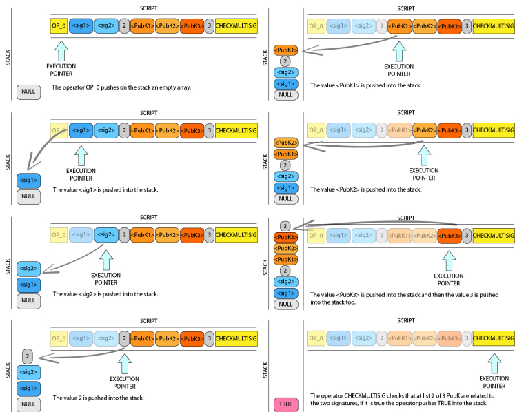
Figure 7: Multi-signature script validation.
