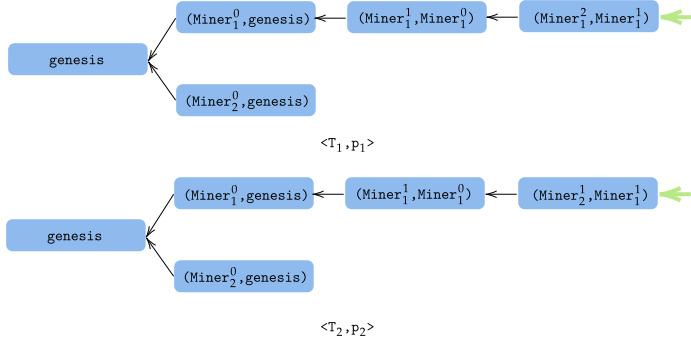
Figure 76: Two ledgers in a state of fork of length 1.
