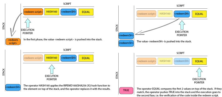
Figure 8: P2SH script validation.
