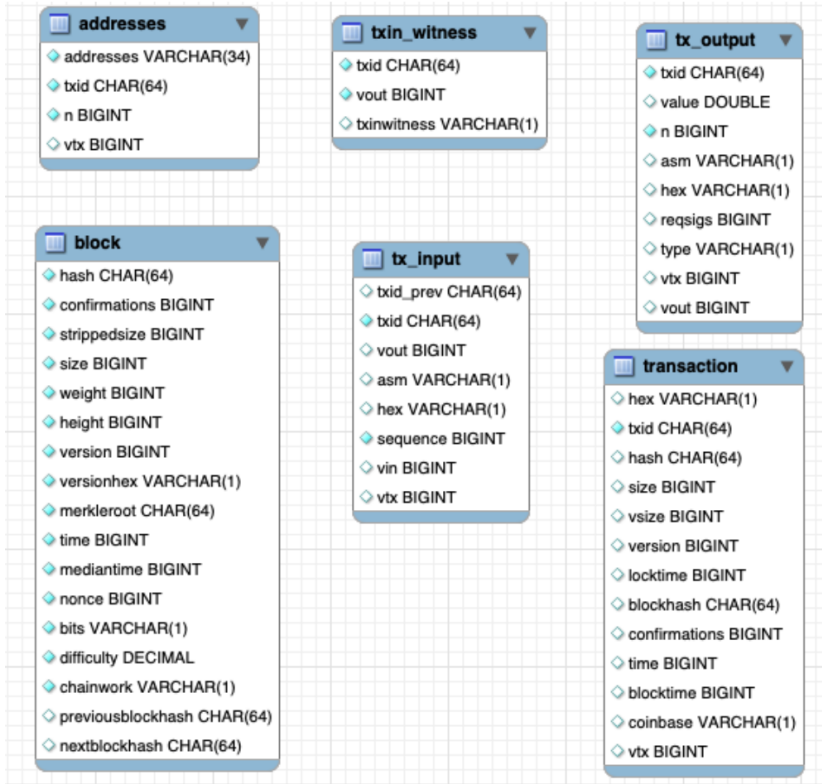
Figure 95: Bitcoin DB schema
