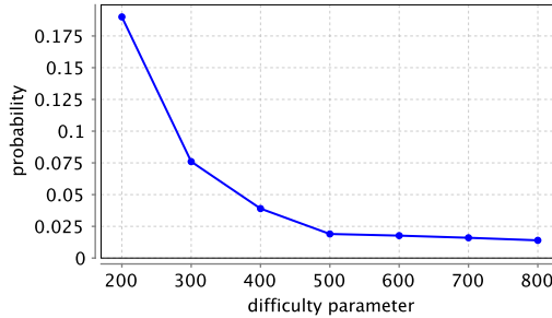
Figure 88: Probability of a fork of length 1 with different difficulty level of the cryptopuzzle; the bound time T is set to 600 seconds.
