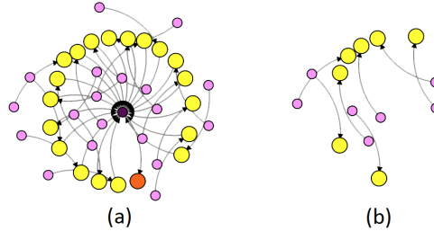
Figure 23: An example (a) of an island as visualised by BlockChainVis. Larger nodes are addresses, and smaller ones are transactions. The darker larger node has a higher (incoming) budget. In (b) we filter (a) by keeping only transactions in the first half of the block interval considered in (a).
