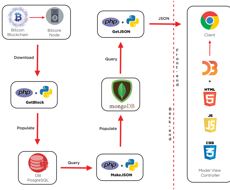
Figure 18: A summary of the architecture and technologies.
