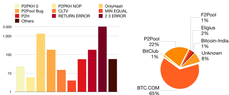
Figure 39: Distribution of non-standard transactions (left) and distribution of their miners (right).
