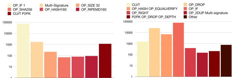
Figure 43: Distribution of OP_IF(left) and non-standard transactions inside P2SH (right).
