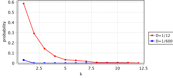
Figure 86: Probability of forks; the bound time T is set to 600 seconds.
