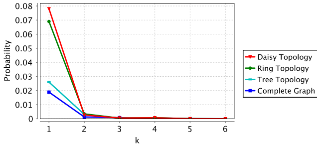
Figure 93: Probability of a fork of length k , the bound time T is set to k * 600 seconds.
