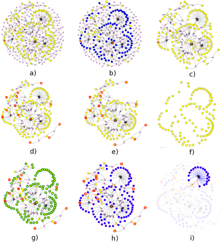
Figure 25: An example of filter application on (a) the initial graph: (b) by highlighting miners, (c) hiding coinbase transactions (rewarding the miners), (d) highlighting leaves, (e) applying a transaction-value interval, (f) showing only roots, (g) visualising paths (most of the two-colour nodes are the same roots in (f), the others are the leaves), (h) combines b and f together (darker nodes highlight the same miners in (b)), (i) focuses on a given transaction.
