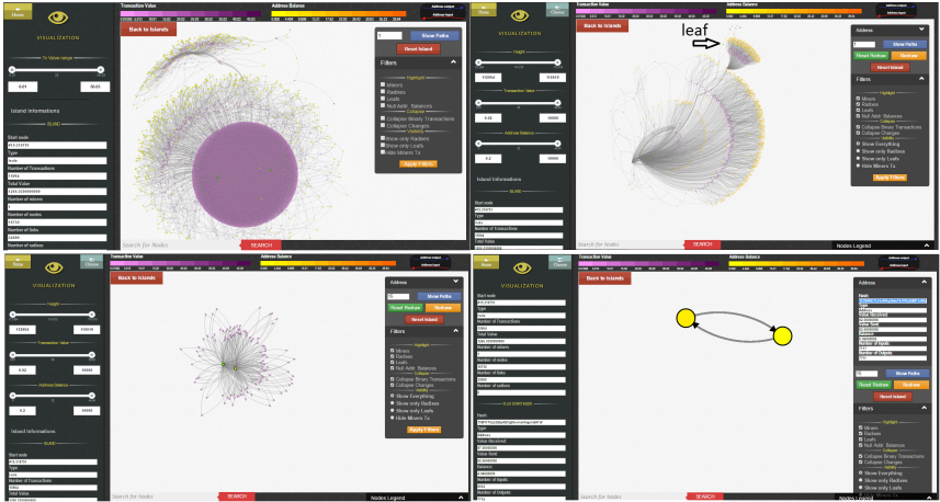
Figure 27: From the full visualisation of an island (top-left), to the only two addresses involved in all the transactions (bottom-right). First, all changes and binary transactions are collapsed to discover a single leaf. Then, all the root-to-leaf paths are extracted.
