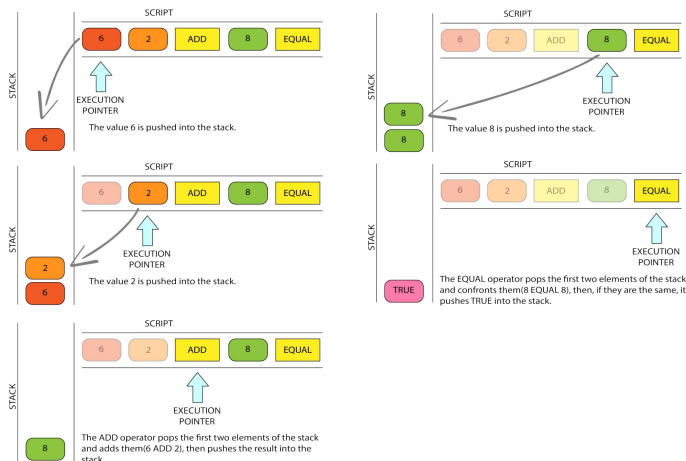
Figure 4: Bitcoin script validation.
