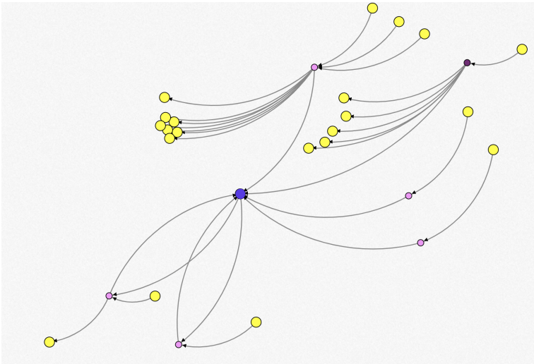
Figure 29: CryptoTorLocker2015 address after (in purple) path filter.
