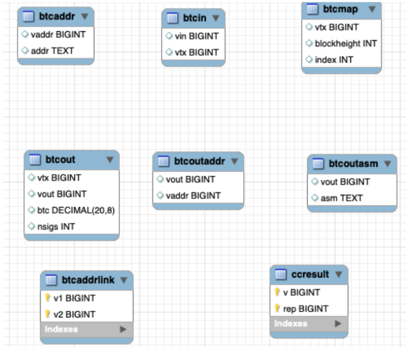
Figure 96: Bitcoin connected components DB schema
