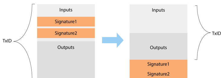
Figure 9: The position of new signatures in witness transactions.
