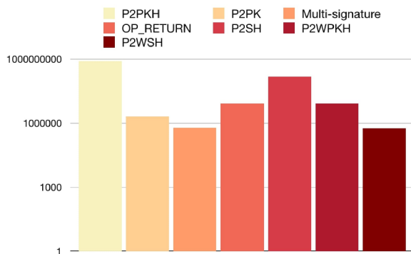
Figure 49: Distribution of transactions in the blockchain.
