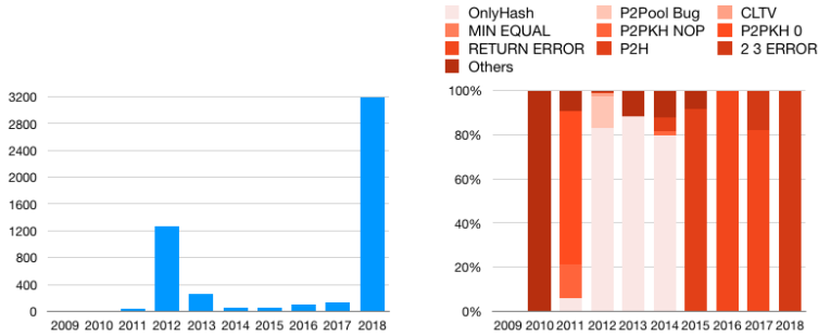
Figure 40: Distribution of non-standard transactions over time (left) and percentage distribution of non-standard transactions type over time (right).
