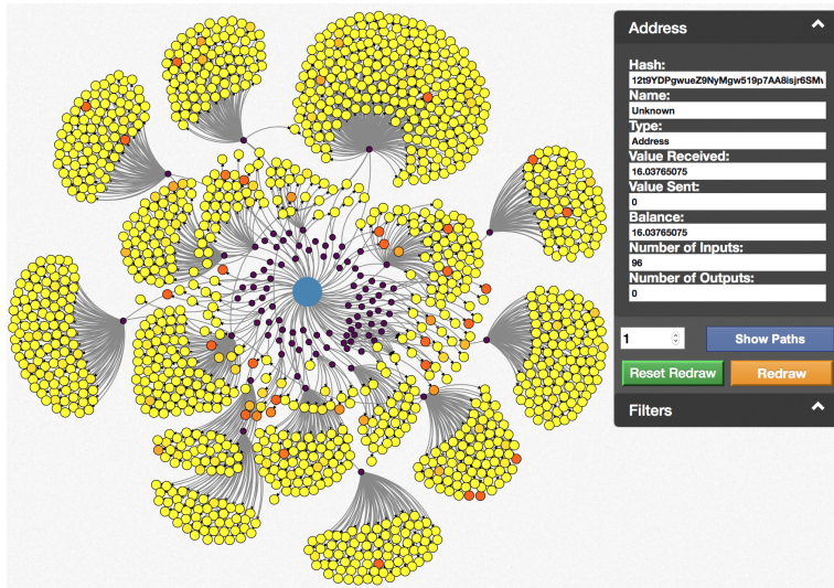
Figure 31: Wannacry address 12t9YDPgwueZ9NyMgw519p7AA8ijsr6SMw income.
