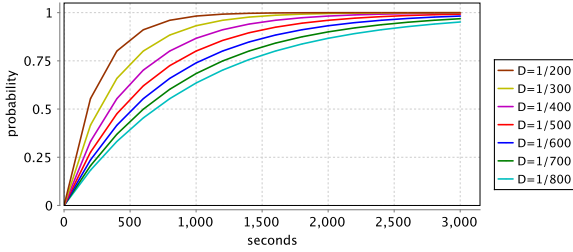
Figure 87: Probability of mining a block within 3000 seconds.
