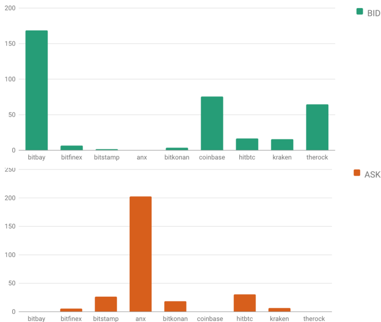
Figure 67: Number of times that BID has been greater and ASK lower.
