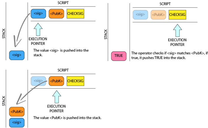
Figure 6: P2PK script validation.
