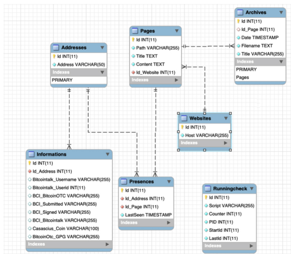
Figure 35: Addresses Scraper DB structure.
