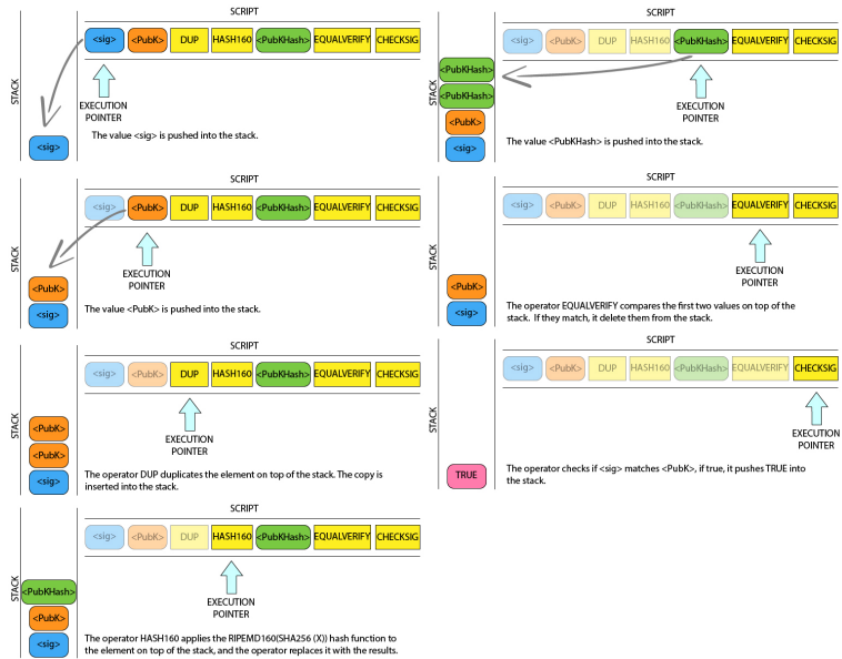
Figure 5: P2PKH script validation.
