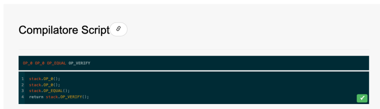
Figure 47: Bitcoin script compiler on Transaction information module.
