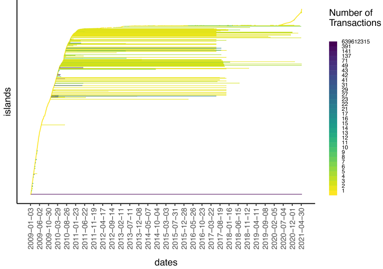
Figure 20: Duration of Bitcoin transaction island.
