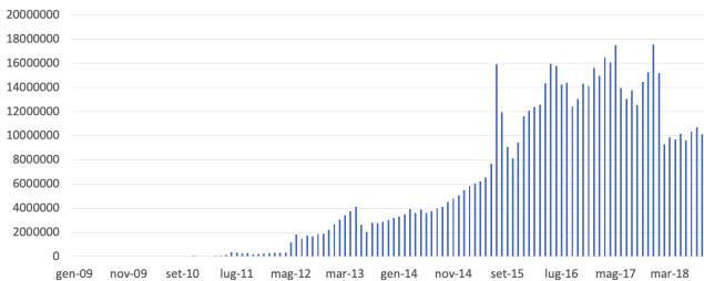
Figure 52: The distribution of address repetitions in time.
