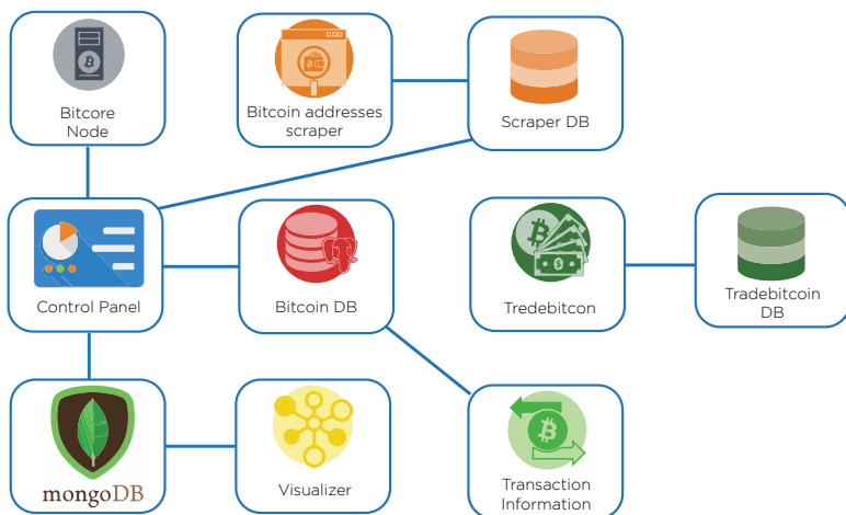
Figure 94: Docker network.
