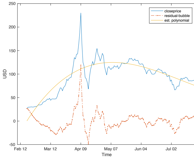
Figure 71: Bitcoin/USD price decomposition
