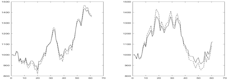
Figure 63: An example with two simulated paths for two months of daily prices: parameters are set to \mu_1 = \mu_2 = 1.5 and \sigma_1 = 0.75 (solid), \sigma_2 = 0.9 (dashed) respectively.
