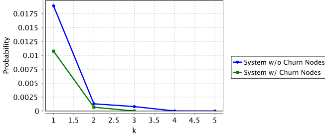
Figure 90: Probability of a fork of length k , the bound time T is set to k * 600 seconds.
