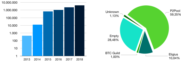
Figure 45: Distribution of OP_RETURN transactions over time (left) and Distribution of miners in “non-standard” OP_RETURN transactions (right).
