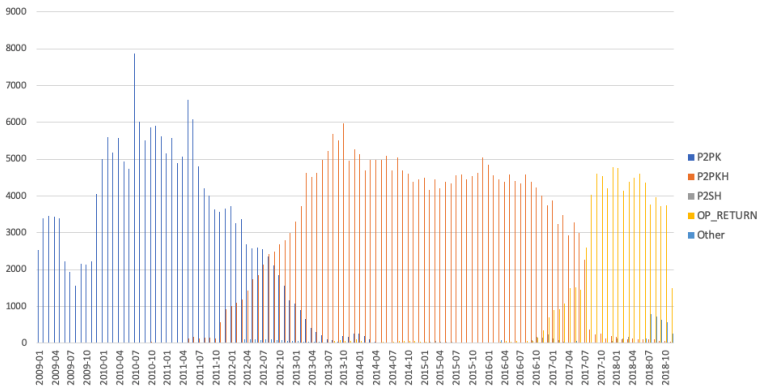
Figure 38: Evolution over time of the output type used in coinbase transactions.
