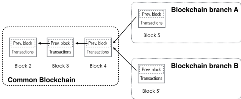
Figure 13: A Fork in Blockchain.
