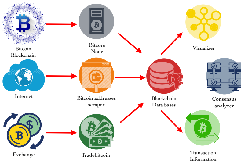
Figure 16: BlockchainVis Suite architecture.
