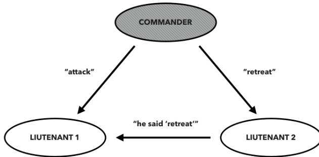
Figure 11: Scenario of the Byzantine Generals Problem where the commander is a traitor.
