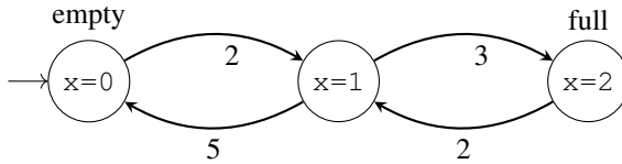
Figure 15: Transition system of module C
