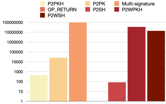
Figure 50: Distribution of transactions inside P2SH ones.
