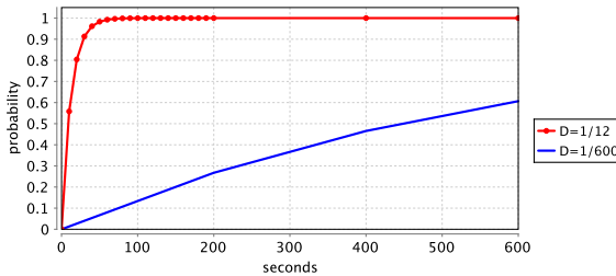
Figure 85: Probability of mining a block within 600 seconds.
