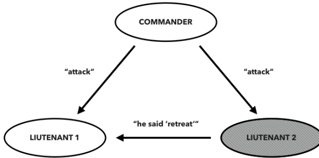
Figure 10: Scenario of the Byzantine Generals Problem where the lieutenant 2 is a traitor.
