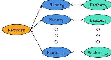
Figure 77: The Bitcoin model architecture.
