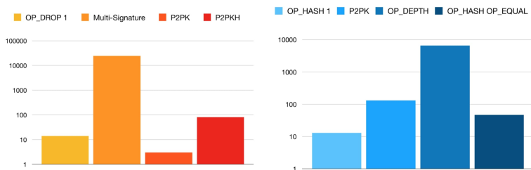
Figure 42: Distribution of OP_DROP (left) and OP_HASH160 OP_EQUALVERIFY transactions inside P2SH (right).
