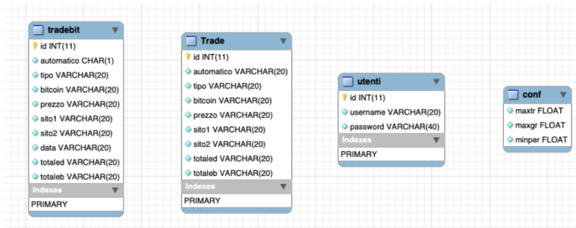
Figure 65: TradeBitcoin DB schema
