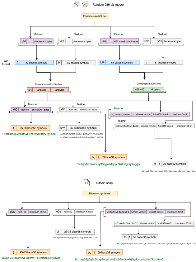
Figure 2: Bitcoin's address generations 1 .
