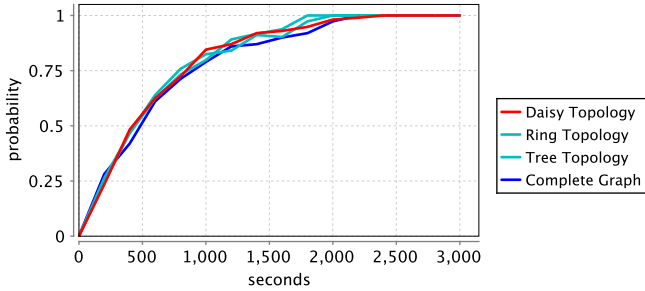
Figure 92: Probability of mining a block within 3000 seconds.
