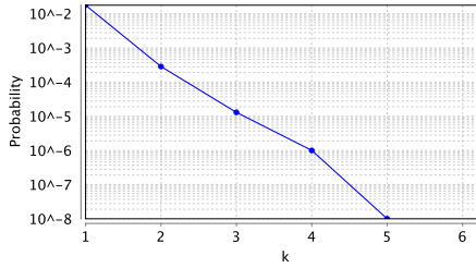
Figure 84: Probability of a fork of length k ; the bound time T is set to k \cdot 600 seconds.
