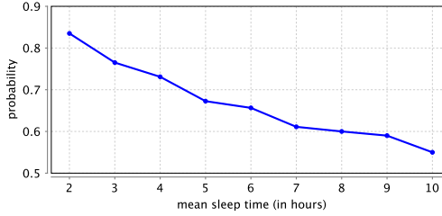
Figure 91: Probability that the node can synchronize in a minute with mean sleep time ranging from 2 to 10 hours.
