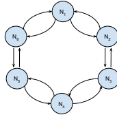
Figure 79: Ring topology.
