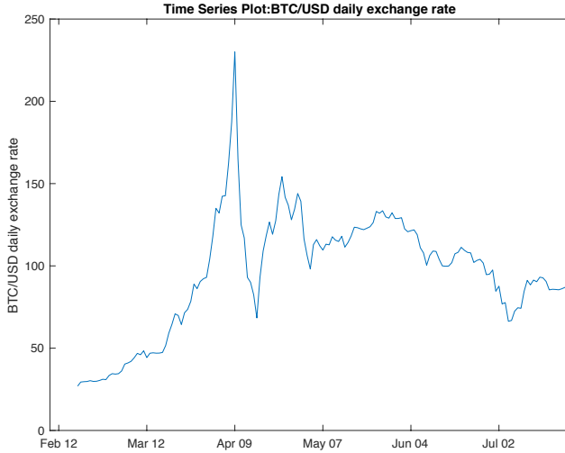
Figure 69: Bitcoin/USD observed time series
