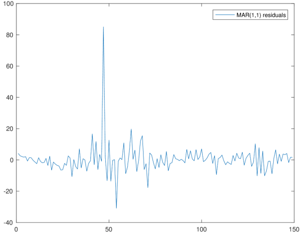
Figure 74: Mixed causal-noncausal MAR(1,1) residuals
