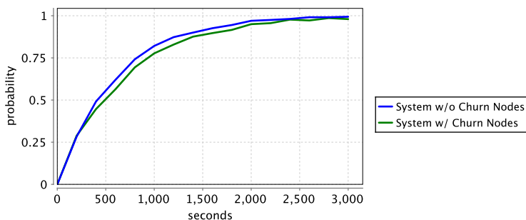
Figure 89: Probability of mining a block within 3000 seconds.
