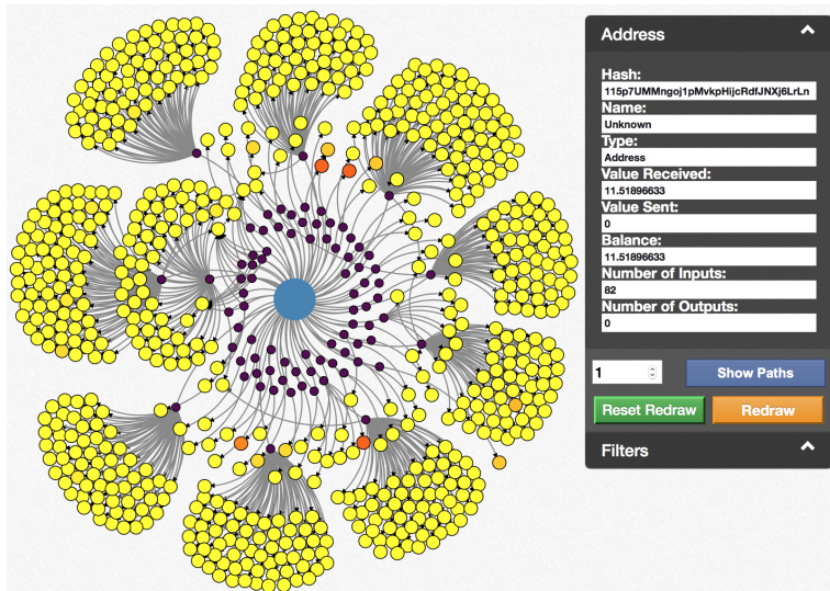
Figure 32: Wannacry address 115p7UMMngoj1pMvvpHjicRdfJNXj6LrLn income.
