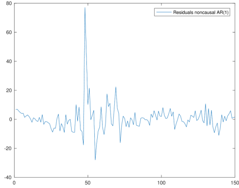
Figure 73: Noncausal AR(1) model residuals
