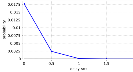
Figure 83: Probability of reaching a fork of length 1 by varying the broadcast delay; the bound time T is set to 600 seconds.
