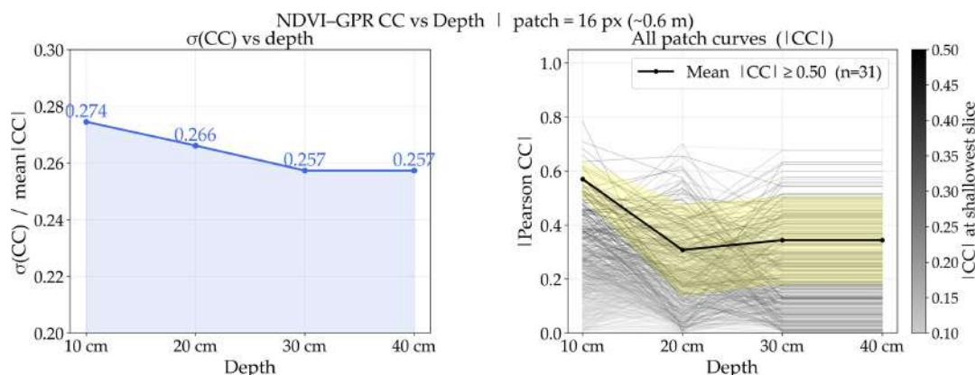
FIGURE 16 | On the left panel, \sigma(CC)/\text{mean}(CC) is represented. The decrease of this trend is a positive indicator that NDVI and GPR data lose correlation in a meaningful way as depth increases. On the right panel, the absolute value of CC is traced against depth. The overall decrease of the signal is indicated by a bold line. Deviations of \pm 1\sigma are shaded in yellow.
