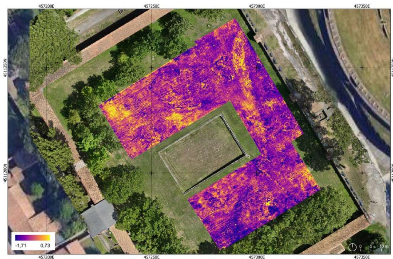
FIGURE 18 | Image-fusion map, enhancing anomalies in [-1.73; 0.73] range of values.
