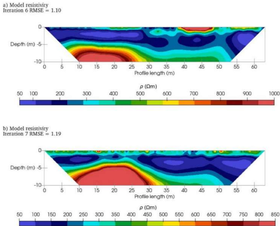
FIGURE 9 | ERT profiles inverted through Resipy. The upper panel displays Section A, whereas Section B is in the lower panel. Resistivity values range from 50 to 1000 \Omega\text{m} in Section A and from 50 to 850 \Omega\text{m} in Section B. High resistivity values are displayed in red, whereas conductive materials are shown in blue.
