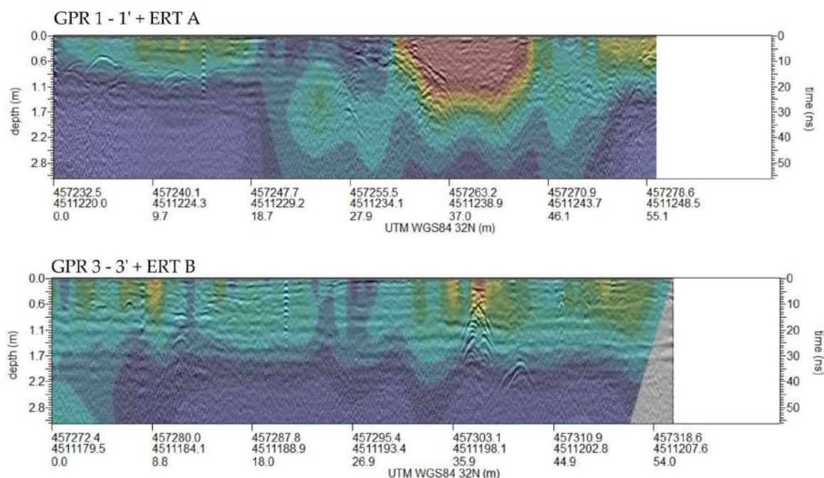
FIGURE 14 | Qualitative integration of ERT and GPR data to enhance and clarify the nature of subsurface features.
