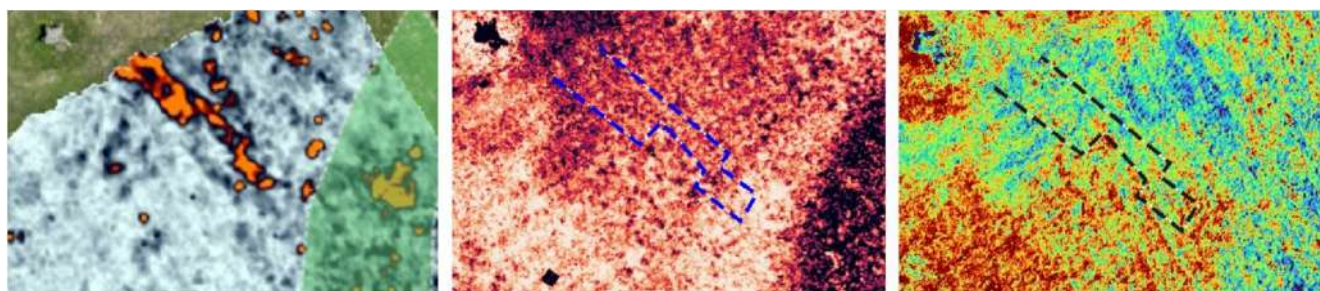
FIGURE 15 | Zoomed-in Area C, illustrating the different detection responses of GPR, NDVI and RN index to the same anomaly, underscoring the methodological variation in anomaly identification.
