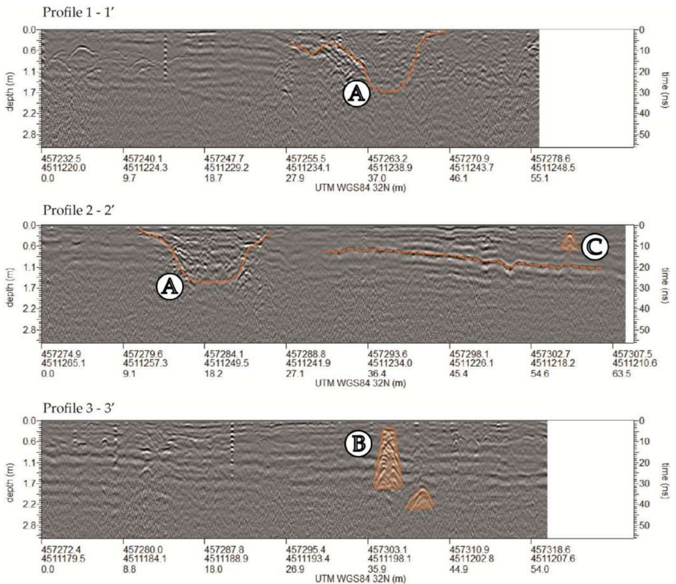
FIGURE 12 | B-scan profiles selected at locations marked in Figure 11. The reflections corresponding to shapes previously noted (A–C) are highlighted in orange.
