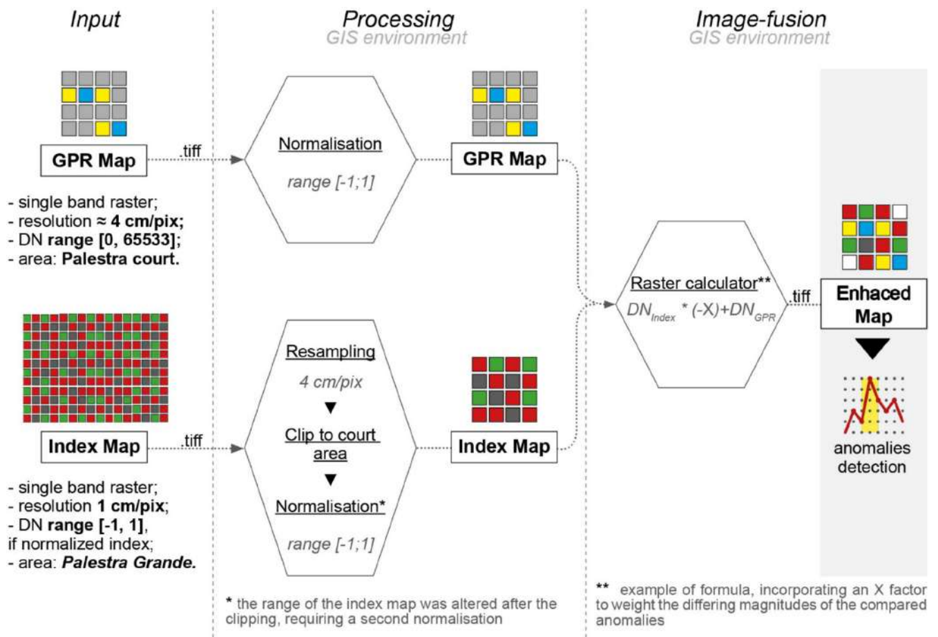
FIGURE 17 | Scheme summarizing the data processing and the final image-fusion map workflow of analysis.
