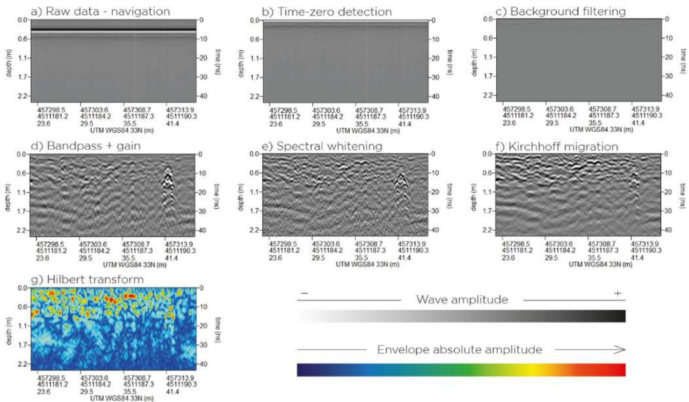
FIGURE 4 | Progressive steps of GPR data filtering on a representative B-scan.
