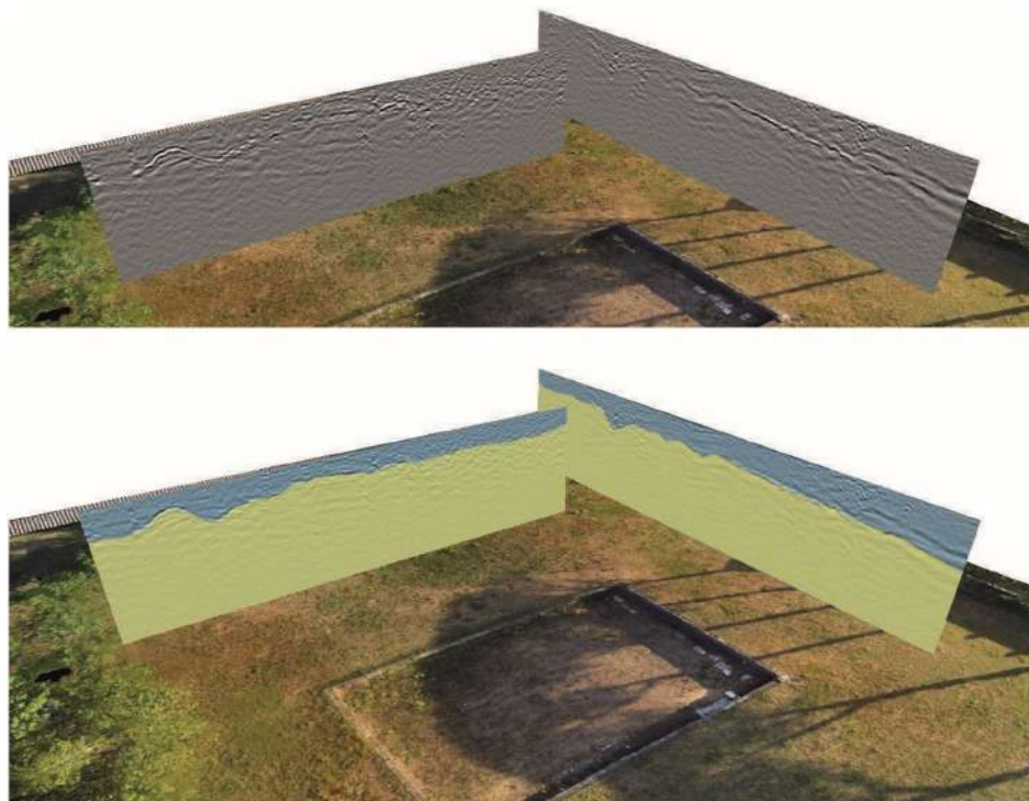
FIGURE 13 | Two representative B-scan sections, which display the layered asset of the subsurface. In the lower panel the same sections are shown with highlighted discontinuities.
