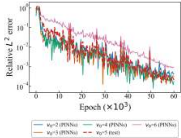
Figure 15: Relative L^2 error of the predicted displacement for the hard-stiffness material without damping.
