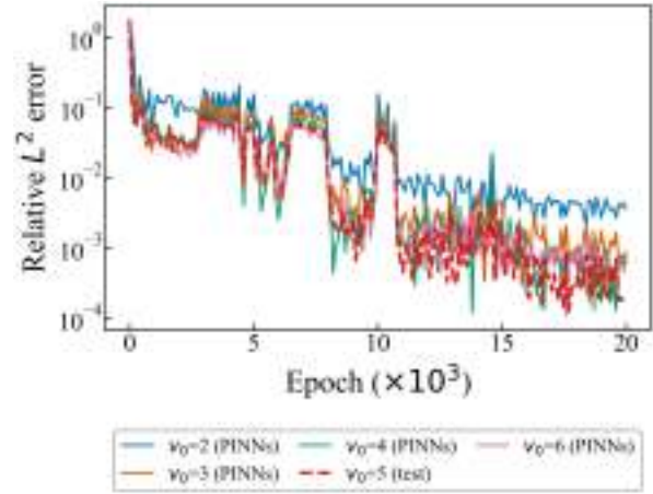
Figure 17: Relative L^2 error of the predicted displacement for the soft-stiffness material with damping.
