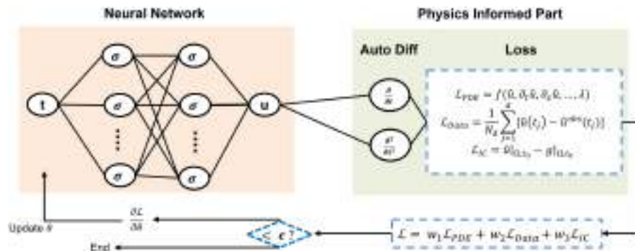
Figure 4: Schematic of the physics-informed neural network (PINN) framework. The neural network maps time to displacement, while automatic differentiation provides the required derivatives to enforce the governing equation. The training is guided by a combined loss incorporating physics, data, and initial condition constraints.
