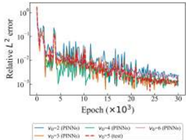
Figure 19: Relative L^2 error of the predicted displacement for the medium-stiffness material with damping.
