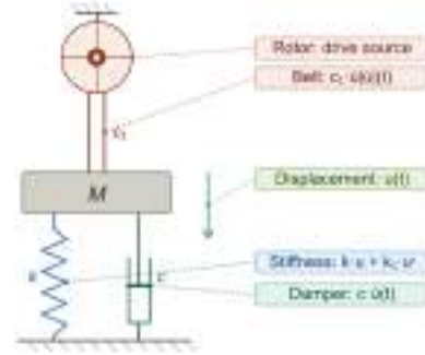
Figure 3: Benchmark System B: Belt–mass system.
