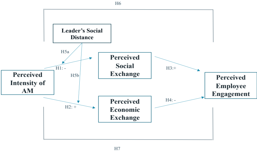
Figure 0-1 Conceptual model
