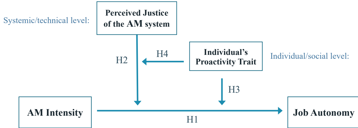
Figure 0-1 Conceptual model
