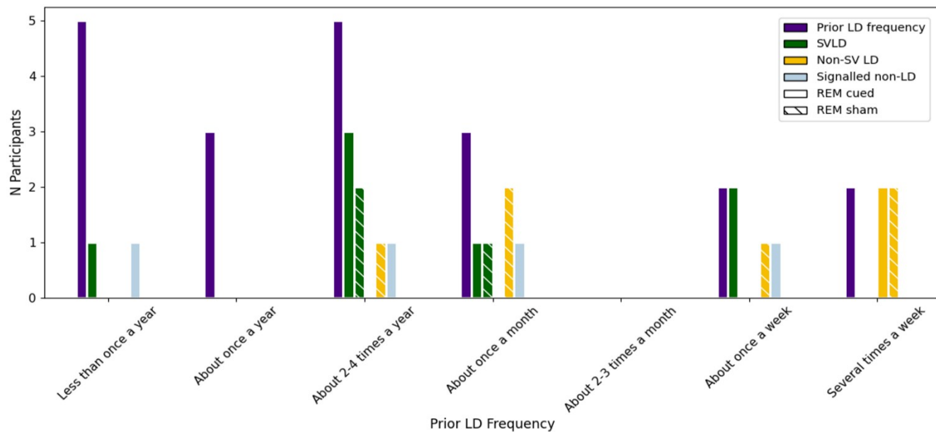
Figure 9. Distribution of dream categories by experimental condition and prior lucid experience.
