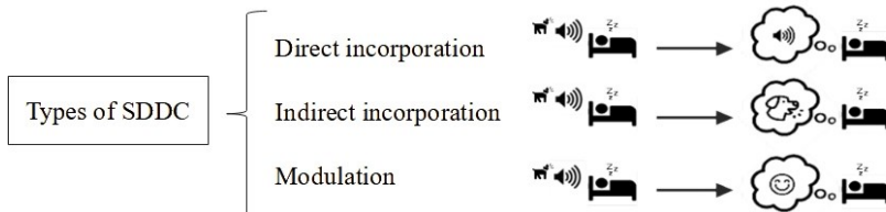
Figure 4. Schematic representation of the main types of stimulus-dependent dream changes (SDDCs) identified in the present review.
