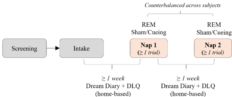
Figure 6. General timeline of the study procedure.
