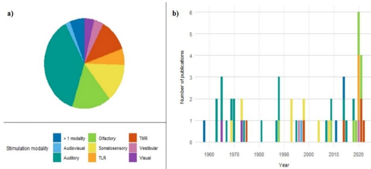
Figure 2. Distribution of selected studies as a function of the targeted sensory modality (a) and year of publication (b).
