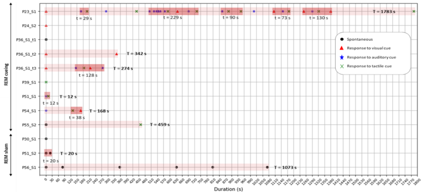
Figure 10. Visualization of signal-verified lucid dream episodes and their estimated duration.
