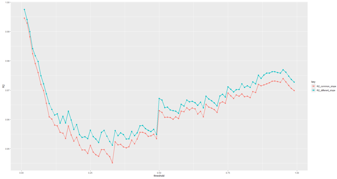
FIG 9. Goodness-of-fit index R^2 of the linear regression on S_{t,h} , in \log_{10} - \log_{10} scale, for each value of the threshold \tau (x-axis). The red line indicates the R^2 obtained imposing a common slope and the blue line the R^2 obtained allowing the slopes to be different across categories. Both the lines are always very close to each other and always higher than 0.95 for any value of \tau .
