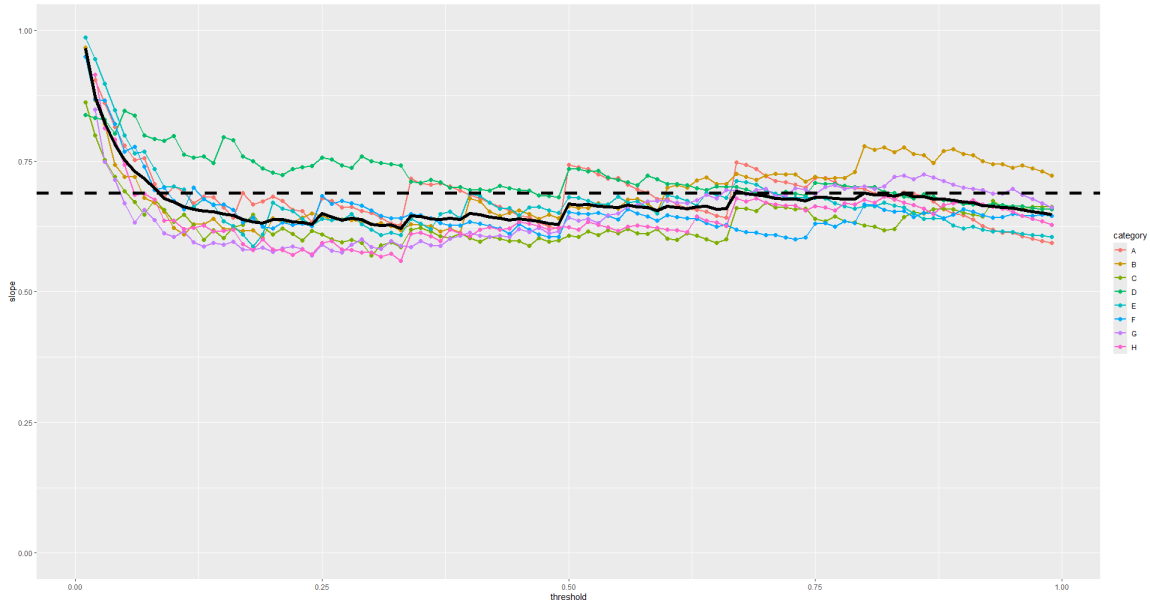
FIG 8. Different slopes estimated through linear regression on S_{t,h} , in \log_{10} - \log_{10} scale, for each category h (color line) and each value of the threshold \tau (x-axis). The solid black line indicates the common slope \hat{\gamma}^* estimated imposing the same slope for all categories. The dashed horizontal black line indicates the common slope \hat{\gamma}^* = 0.689 estimated for \tau = 0.8 in Section 4.
