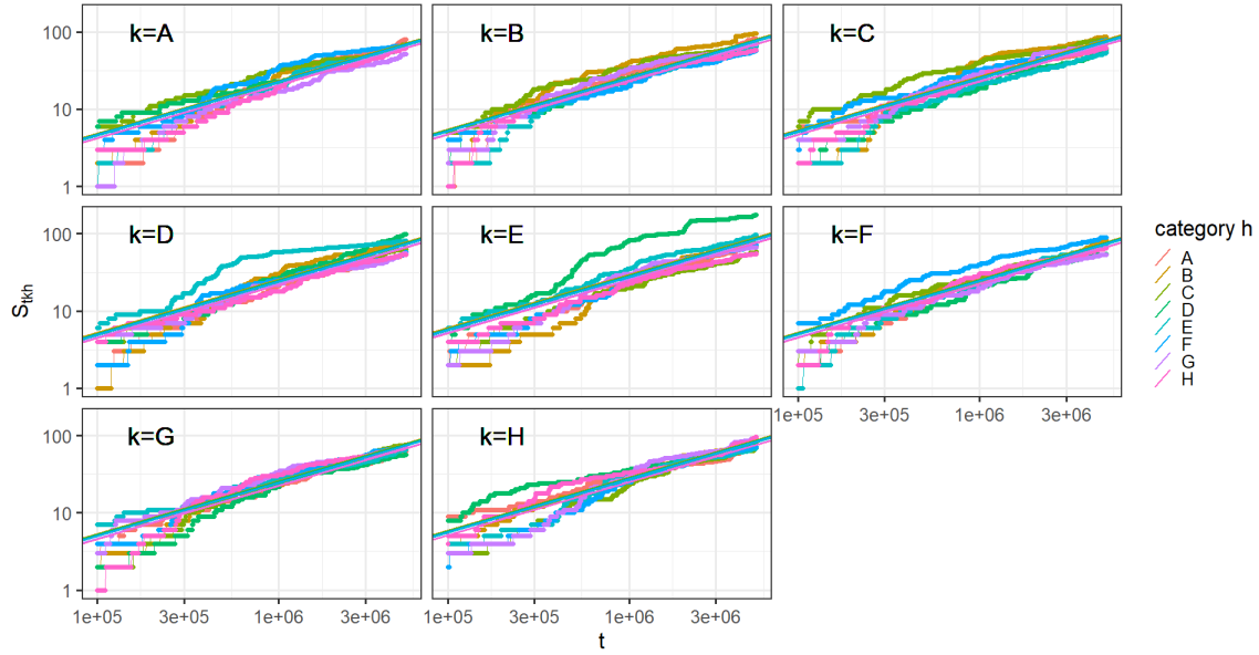
FIG 5. Linear behavior of the successes counter S_{t,k,h} along t in \log_{10} - \log_{10} scale, for each pair (k, h) of categories ( k = sub-figure, h = color). The lines are obtained by a least square interpolation based on a subsample of the dataset with a slope equal to the previously estimated value \hat{\gamma}^* = 0.689 . The goodness of fit R^2 index is 0.851, which is basically the same as the one obtained allowing the slopes to be different across the pairs (k, h) of categories, i.e. 0.855. The common slope suggests one again the presence of interaction across the categories. Moreover, the sub-linear growth reflects a consistent sub-linear scaling of cross-domain innovation flows, suggesting that while knowledge recombination persists, its marginal productivity diminishes over time across all category pairs.
