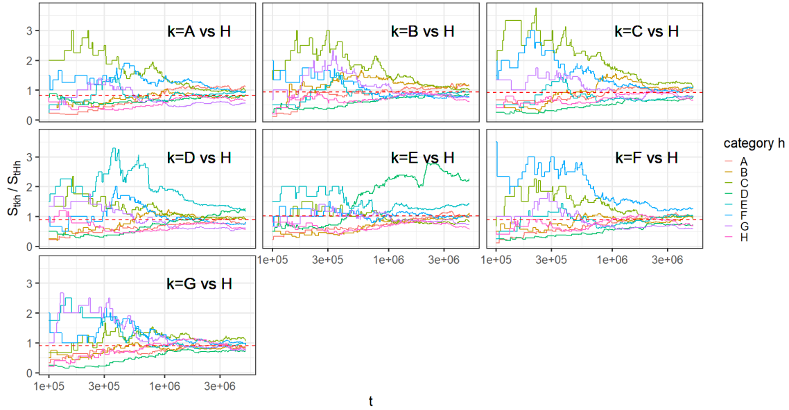
FIG 6. Plot of the process S_{t,k,h}/S_{t,H,h} along time t , for all the pairs (k, h) of categories ( k = sub-figure, h = color), with k \neq H . Category H is arbitrarily chosen to be the baseline category. The horizontal dashed red lines represent the value 10 to the power of the differences between the intercepts of the regression lines in Figure 5 for the pairs of categories (k, h) and (H, h) . This long-run proportionality links early patenting intensity to long-term innovation success, highlighting the path-dependent and self-reinforcing nature of technological trajectories.
