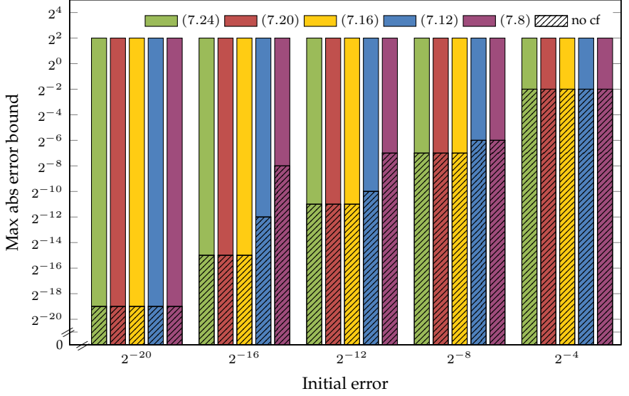
Figure 30: cav10 benchmark: maximum absolute errors.
