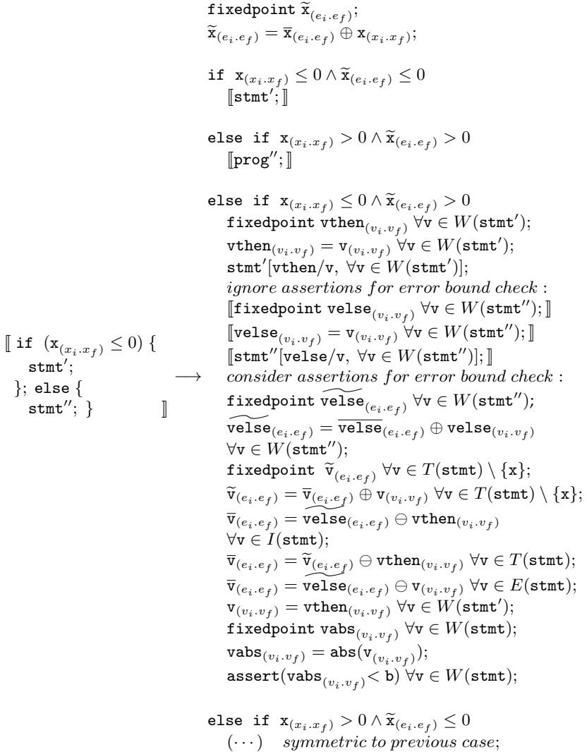
Figure 26: Transformation function \llbracket \cdot \rrbracket : transformation of the if-then-else statement.
