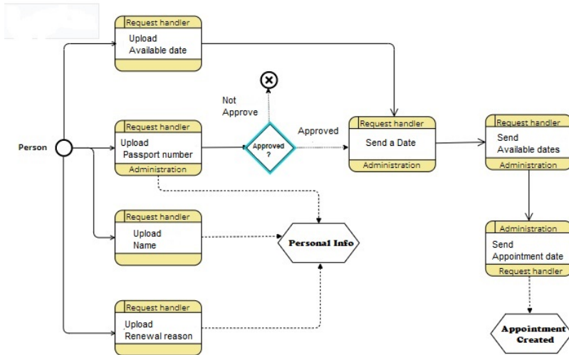
Figure 6: Passport renewal data flow
