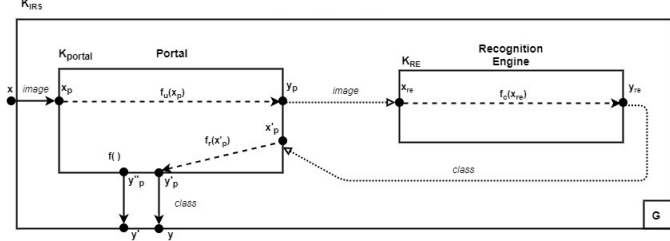
Figure 2: Image Recognition System
