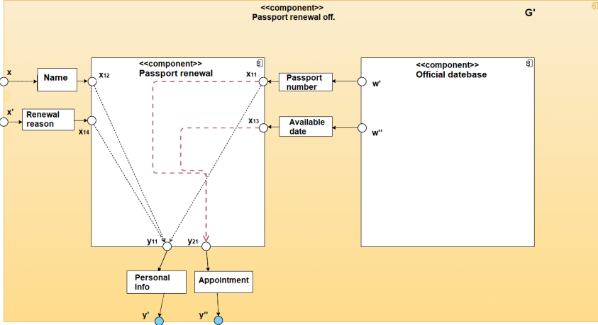
Figure 7: Passport renewal off.
