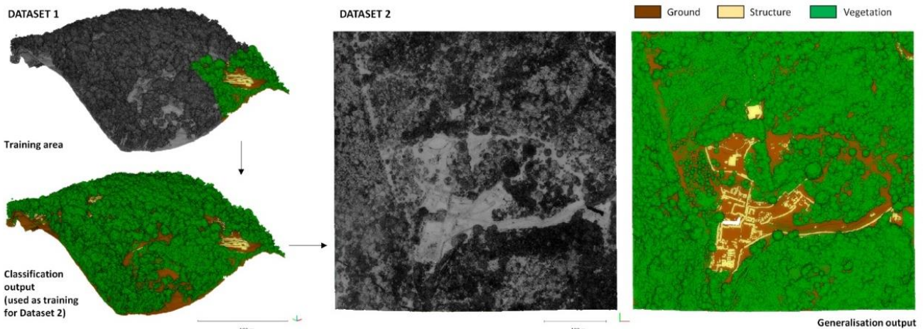
Figure 7. Classification results achieved generalising knowledge acquired in Dataset_1 ( San Martino ai Campi archaeological area) to Dataset_2 ( Roselle archaeological area).
