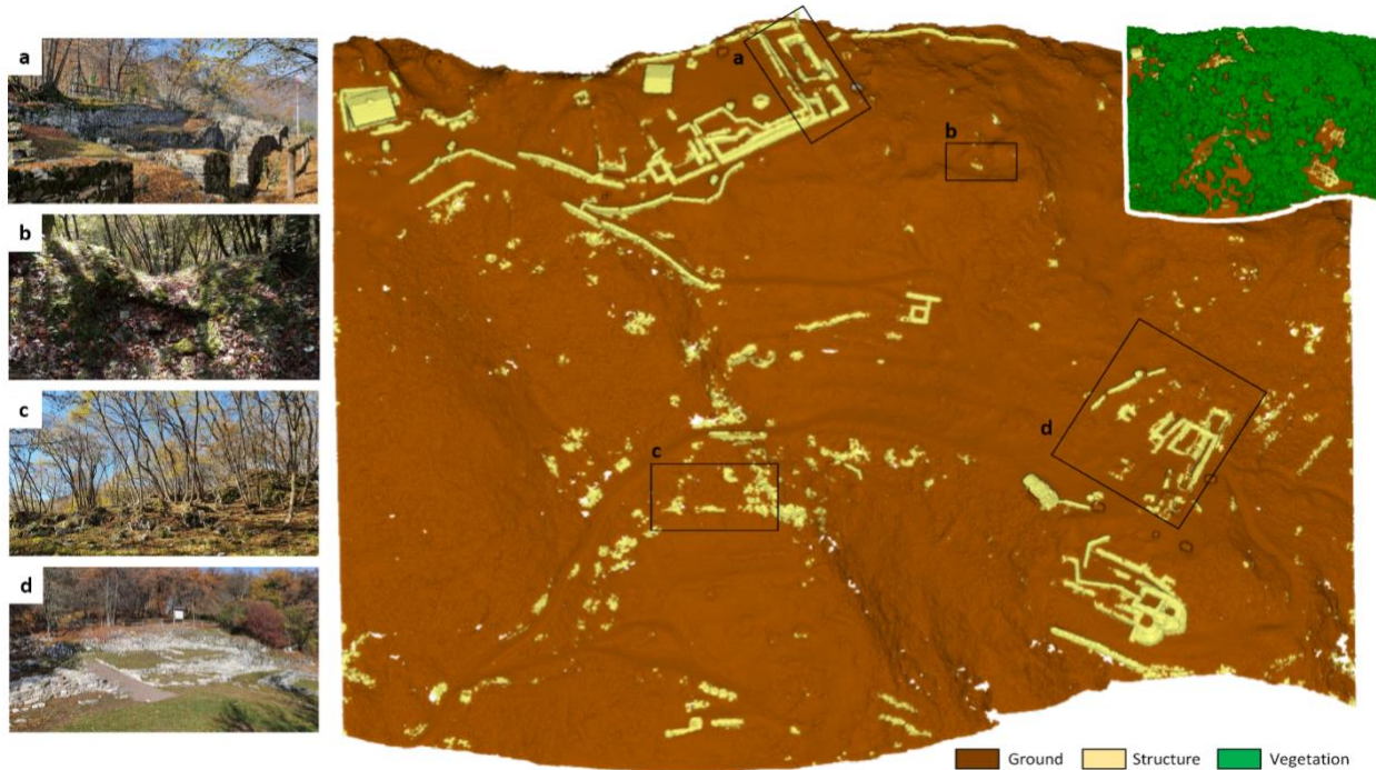
Figure 5. Final semantic segmentation results for Dataset_1 ( San Martino ai Campi archaeological area).
