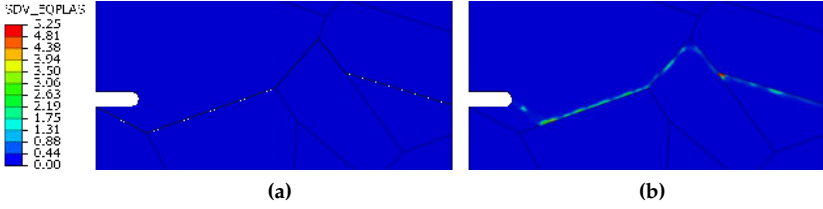
Figure 14: Isocontours depicting the equivalent plastic strain at the end of the analysis for the patterns with a) brittle and b) ductile fracture for the 10-grains benchmark examples.
