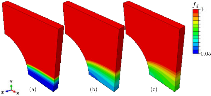
Figure 63: Isocontour plots for the damage function f_d for plates with a hole with different regularisation parameter c_d at u_z = 6.5 mm. In here: (a) c_d = 100 \text{ MPa}^{-1} \text{ mm}^2 , (b) c_d = 500 \text{ MPa}^{-1} \text{ mm}^2 and (c) c_d = 1000 \text{ MPa}^{-1} \text{ mm}^2 .
