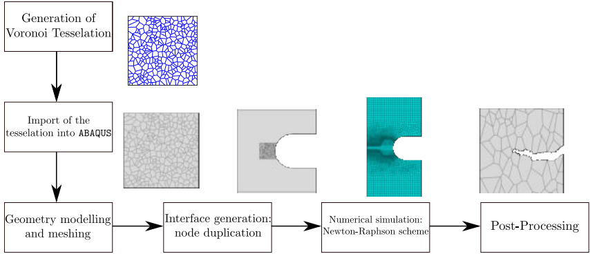
Figure 10: Flowchart that summarises the methodology adopted in the numerical deformation-diffusion-fracture analysis of polycrystalline solids exposed to hydrogen.
