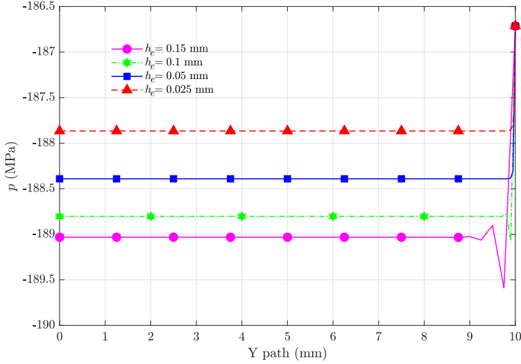
Figure 84: Evolution of the pressure for a vertical path in the sample at x = L - h_e mm for different discretizations at the first increment of the pressure unloading step with a time step of \Delta t = 0.15s . Oscillations in pressure are observed for coarser meshes near the top right corner.
