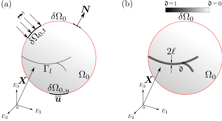
Figure 27: Schematic representation of the two-field large deformation boundary value problem concerning residual stresses: (a) displacement field and (b) phase field parameter for fracture.
