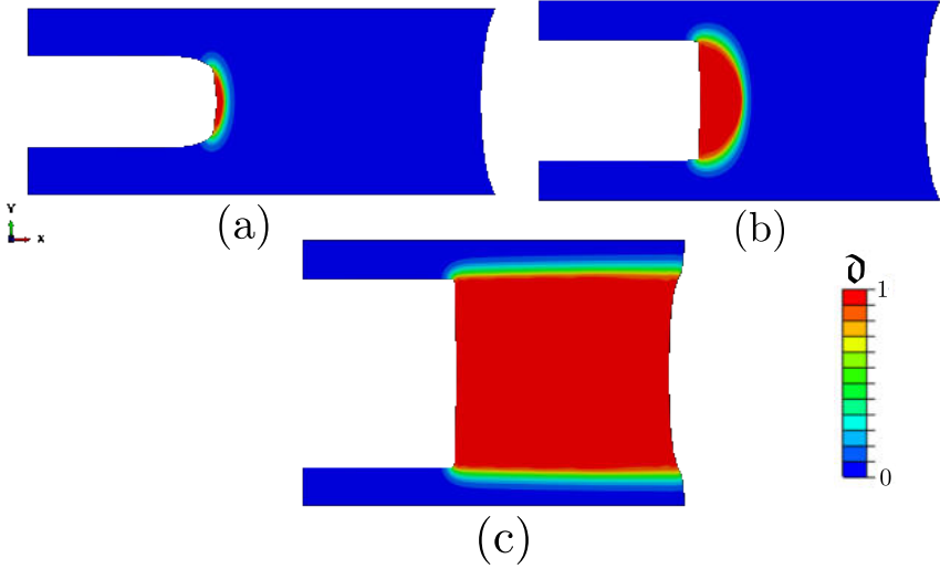
Figure 90: Phase-field isocontours depicting the (a) initiation, (b) propagation and (c) final states in crack propagation of the SENT hydrogel specimen with \lambda_0 = 2.1544 .
