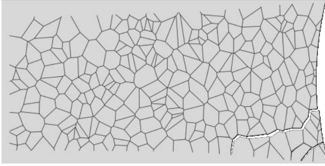
Figure 22: Virtual SSRT experiments on Monel K-500: representative result of intergranular cracking for a sample exposed to an applied potential of E_A = -1.1 V_{SCE} . A crack nucleates at a grain boundary adjacent to the notch tip and then propagates in-between grains towards the centre of the sample.
