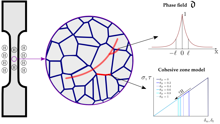
Figure 5: Sketch summarising the modelling framework: the polycrystalline microstructure of metals exposed to hydrogen is explicitly simulated, with the PF method being employed to describe the growth of ductile transgranular cracks while hydrogen-assisted grain boundary decohesion is captured by means of a cohesive zone model. Some of the key variables of the model, that is covered in Chapter 3, are shown; namely, the PF order parameter \vartheta , the PF length scale \ell (governing the size of the interface region), the hydrogen coverage \theta_H , and the cohesive tractions (\sigma, \tau) and separations (\delta_n, \delta_t) .
