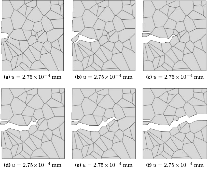
Figure 17: Crack evolution resulting in intergranular fracture for the 50-grain benchmark sample with C = 0.25 wppm sorted by displacement.
