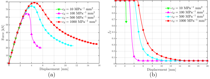
Figure 64: (a) Reaction force-displacement and (b) minimum value of f_d curves for the plate with a hole problem run with a standard spatial CDM approach for different cases of c_d = \{10, 100, 500, 1000\} \text{MPa}^{-1} \text{mm}^2 .
