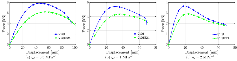
Figure 72: Load-displacement curves for compressible cylindrical shells under bending load conducted with formulations for standard CDM (Q1Q1) and the CDM + EAS (Q1Q1E24) approaches, respectively with different \eta_d .
