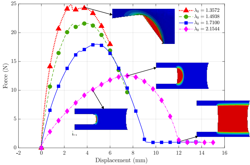
Figure 92: Reaction force-displacement curves for all the conducted SENT hydrogel tests for different initial stretch conditions \lambda_0 . We have included also the micrographs for the evolution of crack fracture along with the instability.
