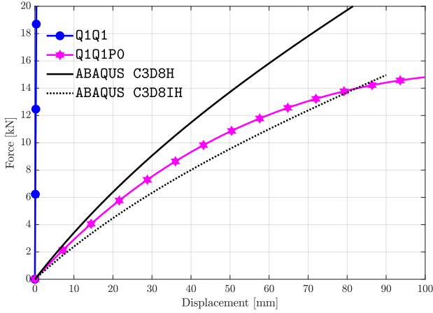
Figure 74: Load-displacement curves for the incompressible cylindrical shell test conducted for Q1Q1 and Q1Q1P0 formulations compared with the ABAQUS hybrid theoretical curves with (C3D8IH) and without considering incompatible modes (C3D8H). The employed saturation parameter has been \eta_d = 0.1 \text{ MPa}^{-1} .
