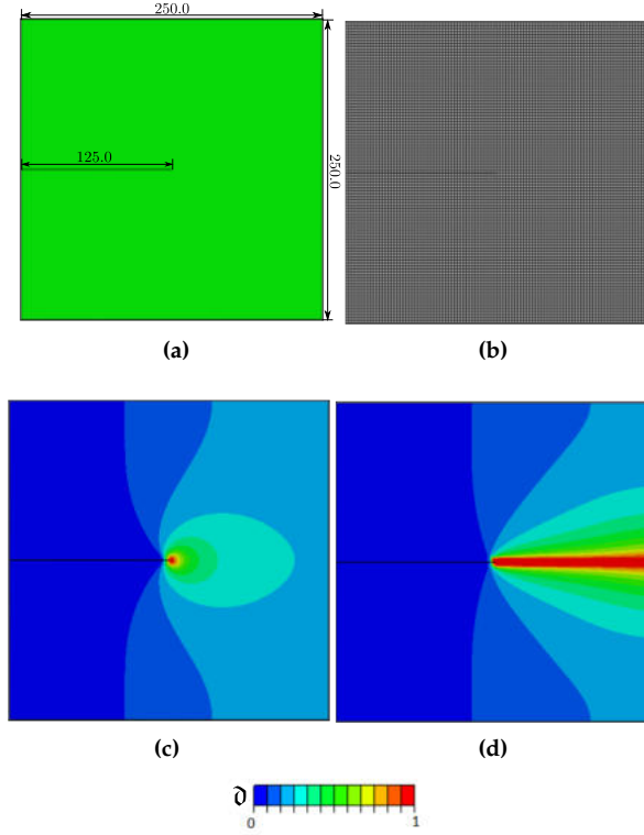
Figure 51: (a) Dimensions in mm, (b) mesh (c) and phase field isocontour for Mode I crack initiation and d) propagation of the single edge notched plate.
