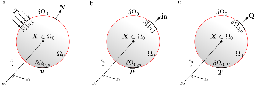
Figure 76: Schematic representation of the three-field boundary value problem: (a) displacement, (b) mass transport, and (c) temperature.
