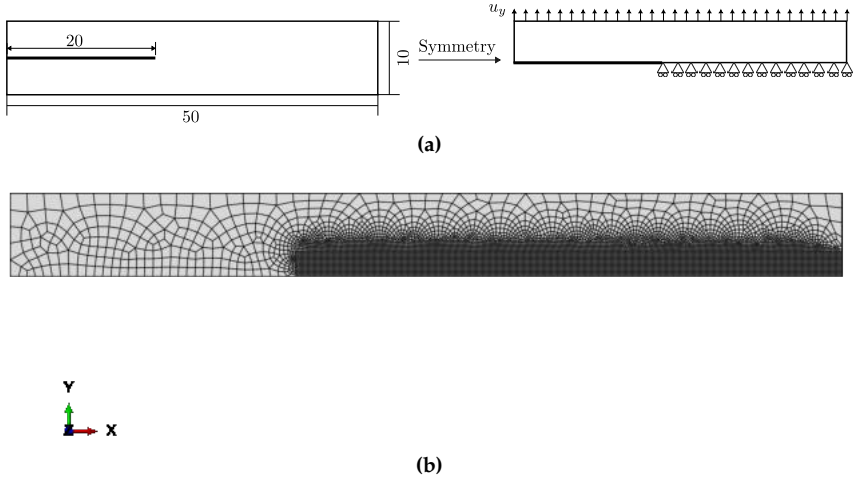
Figure 89: (a) Geometry of the SENT specimen with dimensions in mm; and (b) employed mesh. We depict the full probe and the conducted sample, with symmetry conditions applied.
