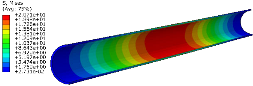
Figure 37: Von Mises stresses distribution associated with a residual stress field in which \bar{\alpha}_d = 500 .
