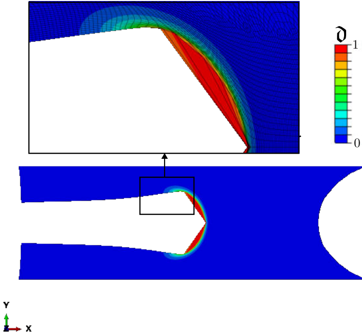
Figure 91: Illustration of the instability due to volumetric locking in the notch tip of the SENT hydrogel with initial stretch \lambda_0 = 1.3572 .
