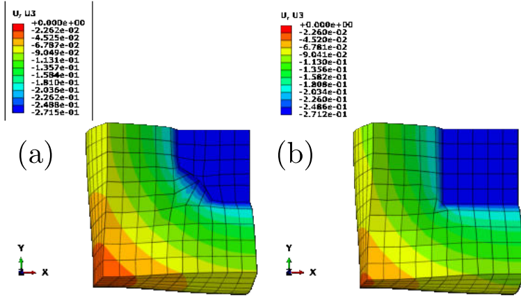
Figure 57: Top view from the deformed of the benchmark problem run with (a) ABAQUS C3D8H and (b) Q1P0 algorithms, respectively. See in (a) the unphysical behavior in the ABAQUS element.
