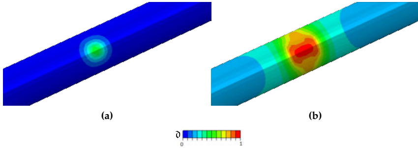
Figure 41: Axial propagation of the phase field parameter for the cylinders with the BC of \vartheta = 0.5 : (a) first step and (b) last load step (axial propagation).
