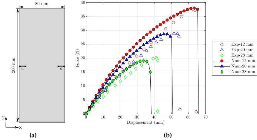
Figure 29: (a) Geometry setup of the double-notched specimen conducted by [248] with (b) the corresponding load-displacement curves (numerical, Num, and experimental, Exp) for verification, precluding viscous effects.
