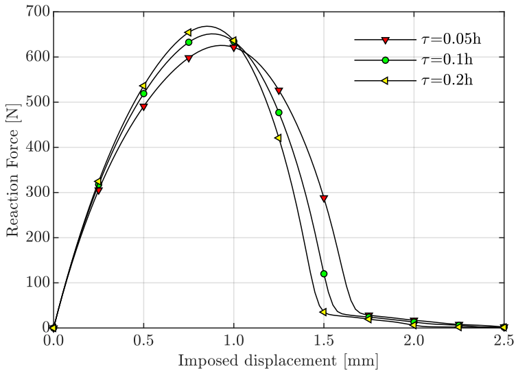
Figure 52: Load-displacement curves for tests of the single-notched square plate with different relaxation times.
