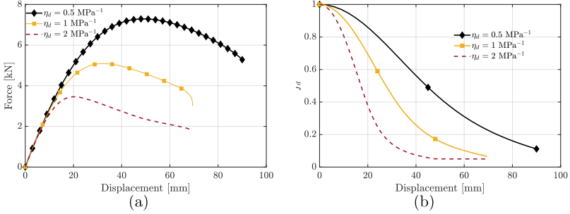
Figure 75: (a) Reaction force-displacement and (b) minimum value of f_d -displacement curves for incompressible cylindrical shells under bending loads conducted with a mixed u-p-J CDM (Q1Q1P0) approach for different cases of \eta_d = \{0.5, 1, 2\} \text{ MPa}^{-1} .
