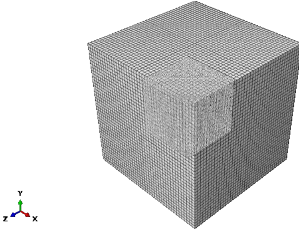
Figure 87: 3-D mesh for the block subject to free swelling: both un-swollen and swollen configurations are represented.
