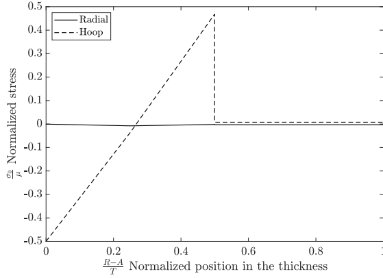
Figure 43: Values of hoop and radial residual stresses along the thickness of the cylinder structure for a path located at Z = L/4 .
