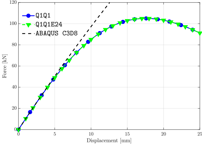
Figure 59: Reaction force-displacement curves for the compressible plate with a hole for the validation probes conducted with a standard CDM (Q1Q1) and CDM + EAS (Q1Q1E24), respectively, compared with ABAQUS C3D8 elements. Employed non-local damage parameters encompass: \eta_d = 0.1 \text{ MPa}^{-1} , \kappa_d = 0 \text{ MPa} and c_d = 1000 \text{ MPa}^{-1} \text{ mm}^2 .
