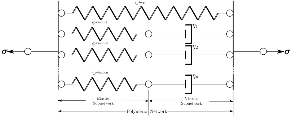
Figure 28: Maxwellian rheological model of the response of the material consisting of the elastic branches, representing the strongly cross-linked network, and the viscous branches, representing the highly mobile with entanglements subnetwork.
