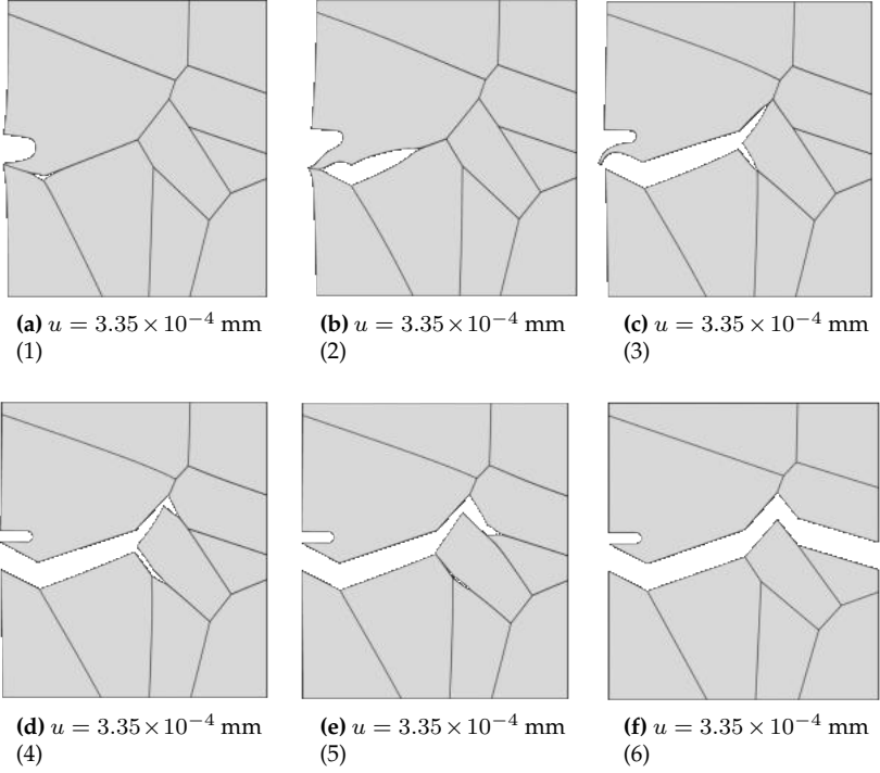
Figure 13: Crack evolution resulting in intergranular fracture for the 10-grain benchmark sample with C = 0.25 wppm sorted by displacement.
