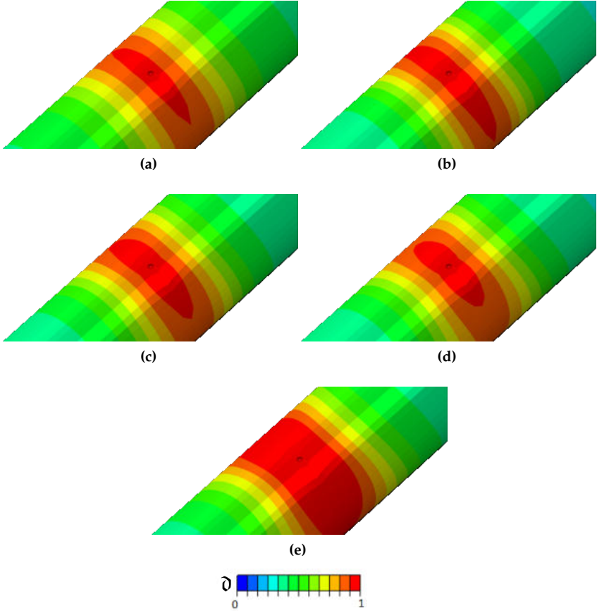
Figure 47: Crack pattern for the different critical Shear Modulus ratios with residual stress parameters \bar{\alpha}_c = 0.5 - \bar{\alpha}_d = 40 . Here displayed (a) G_1/G_2 = 0.2 , (b) G_1/G_2 = 0.5 , (c) G_1/G_2 = 1 , (d) G_1/G_2 = 2 and (e) G_1/G_2 = 5 .
