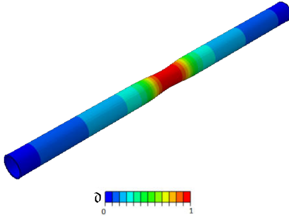
Figure 34: Phase field isocontour at the moment of failure for the non pre-stressed hollow cylinder.
