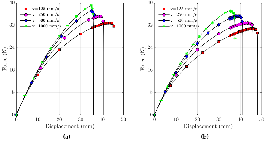
Figure 30: Load-displacement curves for tests with (a) \tau = 0.1 s and (b) \tau = 0.05 s and different displacement rates on the double-notched specimens.
