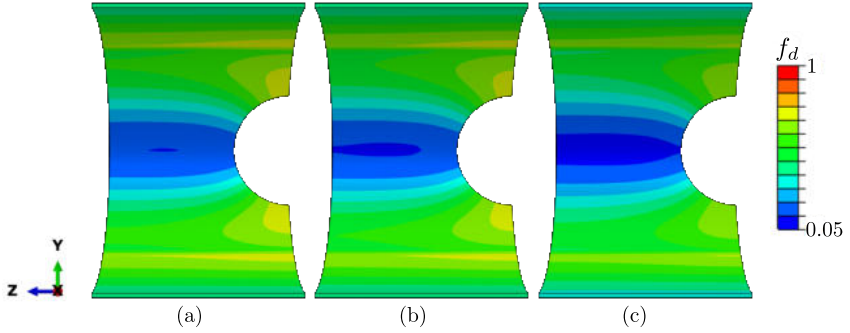
Figure 71: Isocontour plots for the evolution of the damage function f_d for a compressible cylindrical shell under bending load. It has been employed a saturation parameter for damage of \eta_d = 0.5 \text{ MPa}^{-1} for the Q1Q1E24 formulation.
