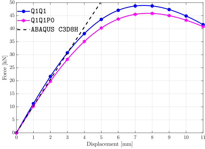
Figure 65: Reaction force-displacement curves for the nearly incompressible plate with a hole for the validation probes conducted with a standard (Q1Q1) and the mixed u-p-J CDM formulations (Q1Q1P0), respectively, compared with ABAQUS C3D8H elements. Employed non-local damage parameters encompass: \eta_d = 0.5 \text{ MPa}^{-1} , \kappa_d = 0 \text{ MPa} and c_d = 1000 \text{ MPa}^{-1}\text{mm}^2 .
