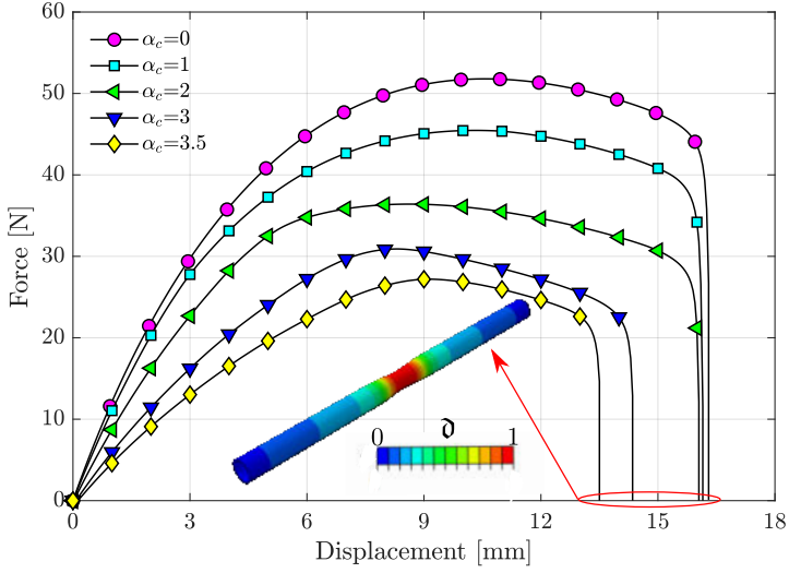
Figure 36: Load-displacement curves for cylinders with different residual stress intensity parameter \bar{\alpha}_c , along with the phase field isocontour in the final step.
