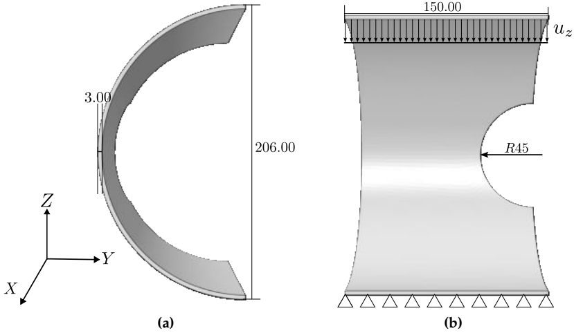
Figure 68: Geometry with boundary conditions and dimensions in mm with (a) profile and (b) frontal view.
