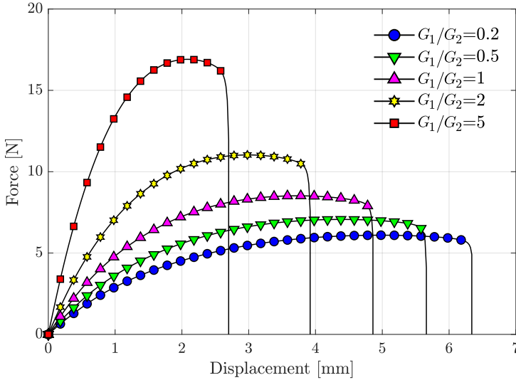
Figure 46: Reaction force-imposed displacement curves for the parametric study changing the shear modulus ratio with residual stress parameters \bar{\alpha}_c = 0.5 - \bar{\alpha}_d = 40 .
