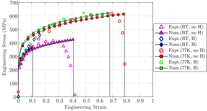
Figure 25: Role of temperature on the failure of polycrystalline Ni samples: engineering stress-strain curves for both H-charged and non-charged samples pulled to failure at 77K and at ambient temperature (298 K).
