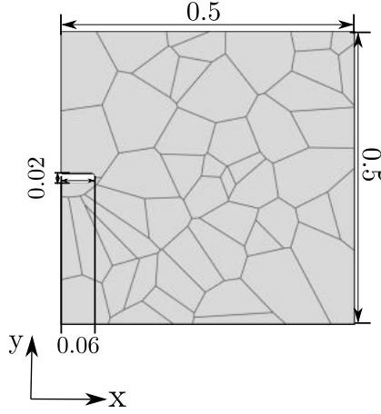
Figure 11: Geometry for the 50-grained SENT place with dimensions in mm.
