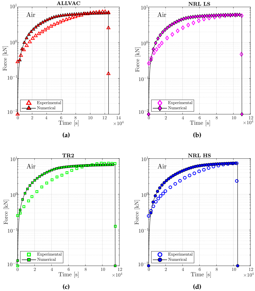
Figure 21: Virtual SSRT experiments on Monel K-500: numerical and experimental force versus time curves obtained in the absence of hydrogen for each material lot; namely, (a) Allvac, (b) NRL LS, (c) TR2 and (d) NRL HS.
