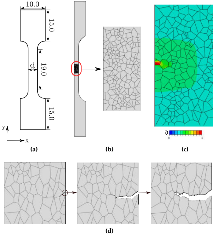
Figure 24: Role of temperature on the failure of polycrystalline Ni samples: (a) geometry with dimensions in mm, where d = 4 mm for 77 K and d = 3.6 mm for RT specimens [86], (b) augmented view of the microstructure region, with 200 grains, (c) ductile (transgranular) damage, as predicted by the phase field, and (d) intergranular crack nucleation and growth, as assisted by hydrogen. Representative results shown from calculations at ambient temperature.
