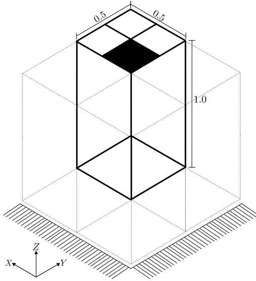
Figure 54: Scheme for the block under compressive load modelled. The area in bold corresponds with the region where the compressive u_z is applied on. The dimensions are given in mm. Dotted lines correspond to the regions generated by symmetry.
