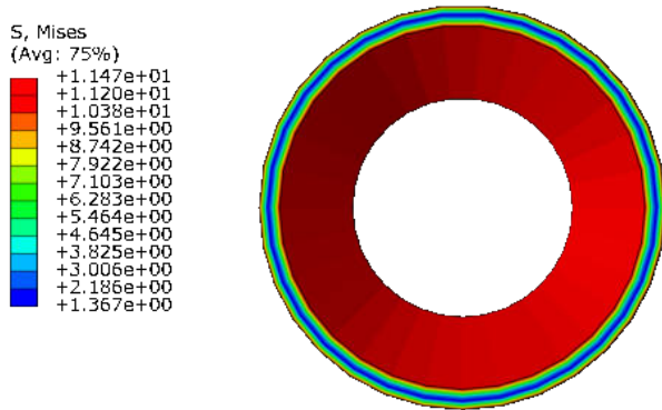
Figure 35: Von Mises stresses distribution for a residual stress with \bar{\alpha}_c = 1 .
