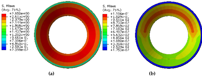
Figure 44: Von Mises stress isocontour for (a) the inner and (b) the outer layer, respectively, for a pre-stressed bi-layered cylindrical structure.
