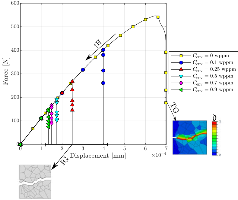
Figure 18: Predicted force versus displacement curves for the 50-grain SENT benchmark. The results are presented as a function of the environmental hydrogen concentration C_{\text{env}} , and images are embedded to showcase the different intergranular (IG) and transgranular (TG) cracking patterns observed.
