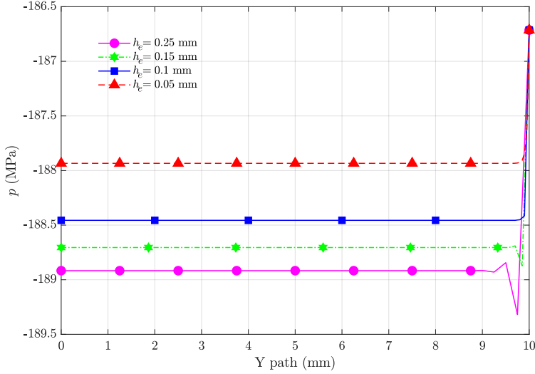
Figure 82: Evolution of the pressure for a vertical path in the sample at x = L - h_e mm for different discretizations at the first increment of the pressure unloading step with a time step of \Delta t = 0.5 s. Oscillations in pressure are observed for coarser meshes near the top right corner.
