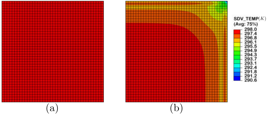
Figure 85: Isocontour displaying the temperature field (a) without and (b) with considering the fluid flow and elastic stretching influence on the temperature.
