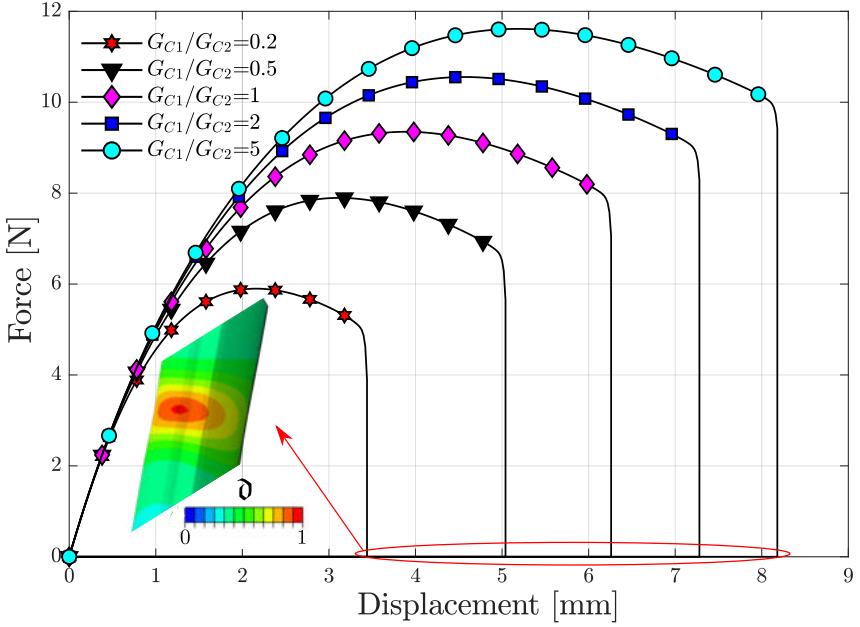
Figure 48: Reaction force-imposed displacement curves for the parametric study changing the critical energy release rate ratio without residual stress.
