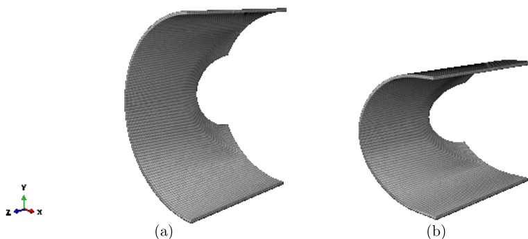
Figure 69: Cylindrical shell: undeformed and deformed configuration.
