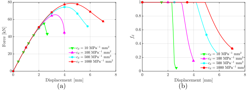
Figure 67: (a) Reaction force-displacement and (b) minimum value of f_d -displacement curves for the nearly incompressible plate with a hole problem run with a mixed u-p-J CDM (Q1Q1P0) approach for different cases of c_d = \{10, 100, 500, 1000\} \text{ MPa}^{-1} \text{ mm}^2 .
