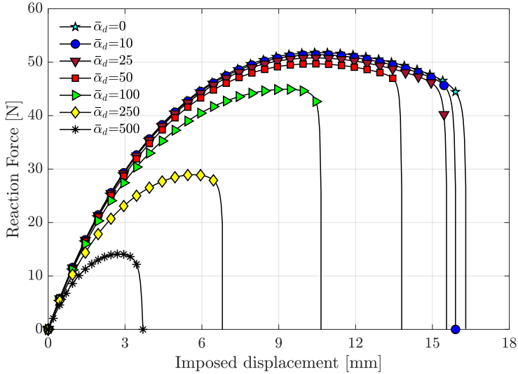
Figure 38: Load-displacement curves for cylinders with different residual stress intensity parameters \bar{\alpha}_d .
