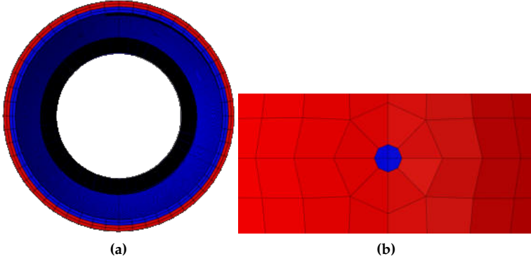
Figure 42: (a) Isometric and (b) zoomed-in-the-notch view of the cylindrical structure with two layers, distinguishing the layer by the color.
