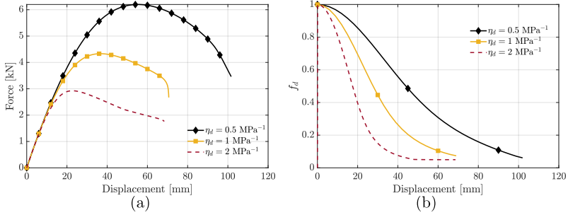
Figure 73: (a) Reaction force-displacement and (b) minimum value of f_d -displacement curves for compressible cylindrical shells under bending loads conducted with a CDM + EAS (Q1Q1E24) approach for different cases of \eta_d = \{0.5, 1, 2\} \text{ MPa}^{-1} .
