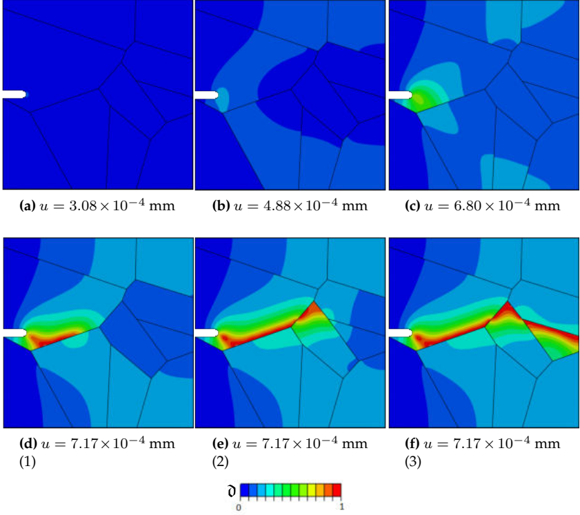
Figure 12: Crack evolution resulting in transgranular fracture for the 10-grain benchmark sample with C = 0 wppm sorted by displacement. Plotted is the phase-field parameter.
