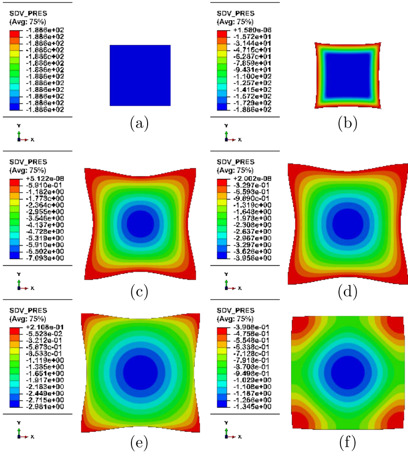
Figure 79: Steps of the swelling-deswelling process: states for (a) 0 s, (b) 300 s, (c) 12 h, (d) 24 h, (e) 25 h and (f) 49 h. Represented within this plots is the solvent pressure p .
