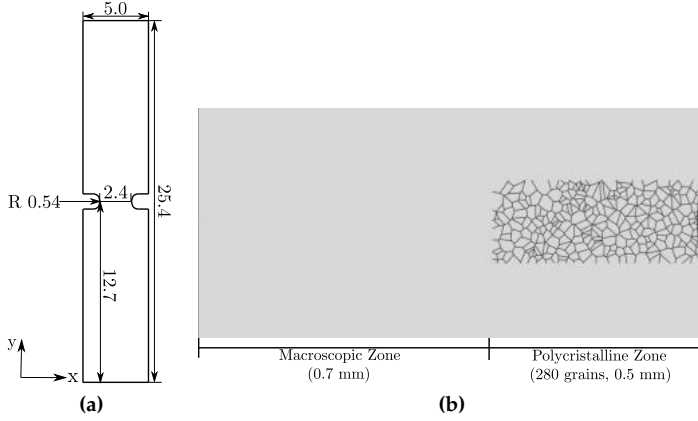
Figure 19: Virtual SSRT experiments on Monel K-500: (a) geometry of the specimens, with dimensions in mm, and (b) augmented view of the region ahead of the notch, showcasing the division between macroscopic and microscopic regions.
