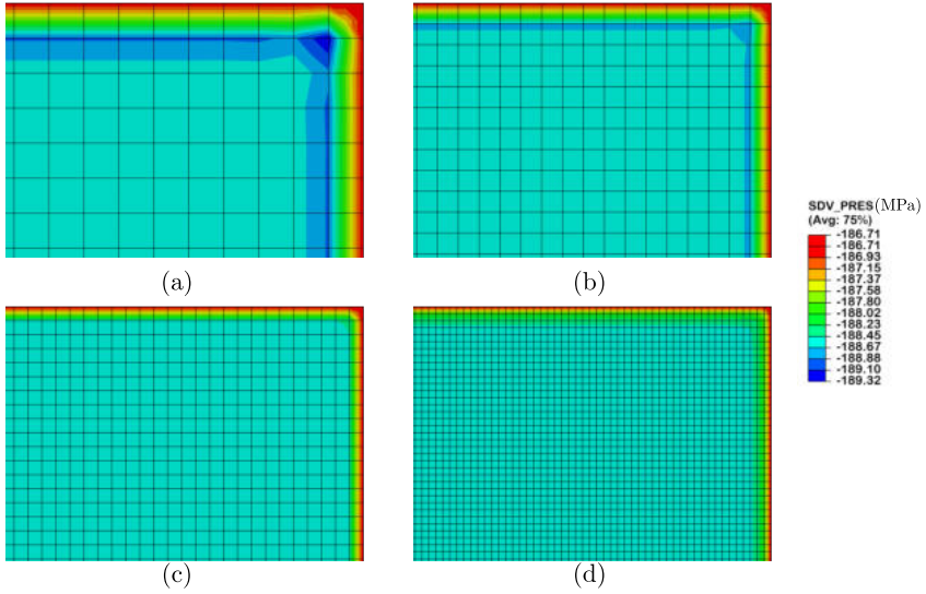
Figure 81: First increment of unloading pressure ramps conducted for discretizations with element sizes: (a) h_e = 0.25 , (b) h_e = 0.15 , (c) h_e = 0.1 and (d) h_e = 0.05 mm with a time step of \Delta t = 0.5 s. It is observed how by increasing discretization, the variation of the pressure becomes smooth.
