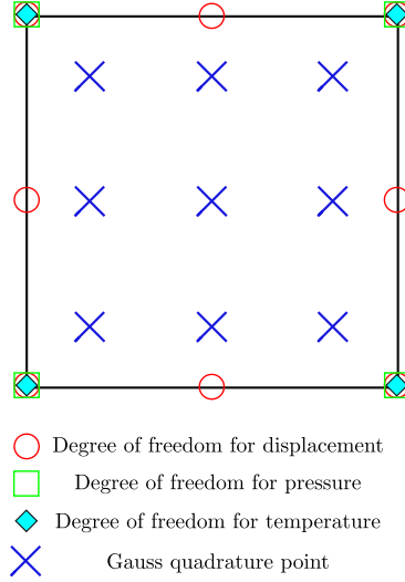
Figure 77: 2-D illustration of a u - p - T mixed finite element, displaying the degrees of freedom and the Gauss quadrature points. 8-node biquadratic element is used for the displacement while 4-node bilinear quadrilateral elements are utilized for pressure and temperature.
