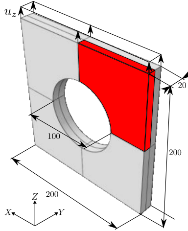
Figure 58: Geometry and BCs for the plate with a hole. The dimensions are in mm, and only an eighth of the sample is modelled, the region in red.
