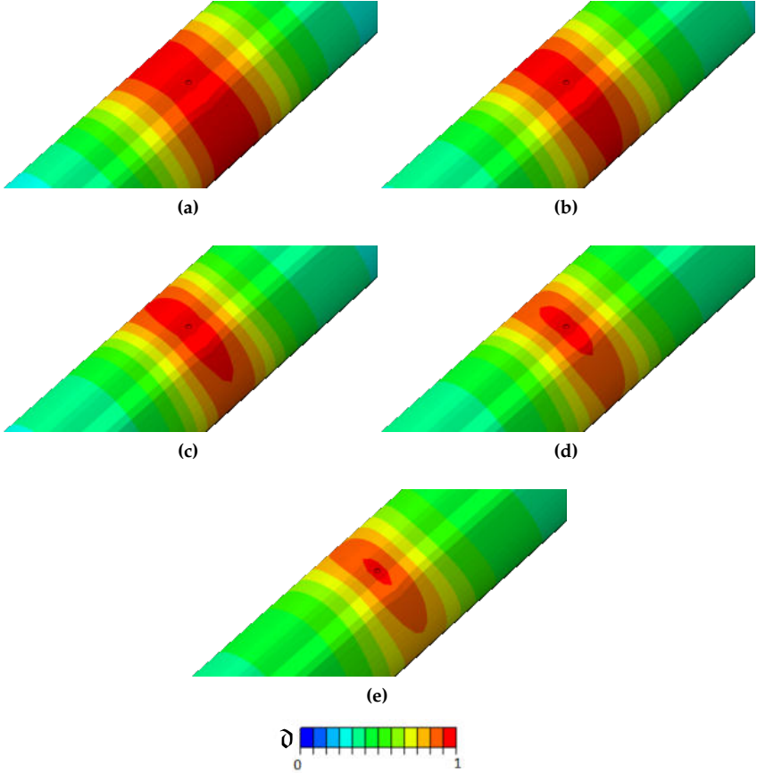
Figure 50: Crack pattern for the different critical energy release rate ratios with residual stress parameters \bar{\alpha}_c = 0.5\text{-}\bar{\alpha}_d = 40 . Here displayed (a) \mathcal{G}_{C1}/\mathcal{G}_{C2} = 0.2 , (b) \mathcal{G}_{C1}/\mathcal{G}_{C2} = 0.5 , (c) \mathcal{G}_{C1}/\mathcal{G}_{C2} = 1 , (d) \mathcal{G}_{C1}/\mathcal{G}_{C2} = 2 and (e) \mathcal{G}_{C1}/\mathcal{G}_{C2} = 5 .
