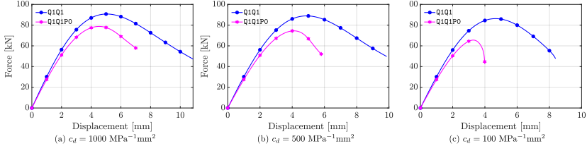
Figure 66: Reaction force-displacement curves for the compressible plate with a hole problem comparing standard CDM (Q1Q1) and mixed u-p-J + CDM (Q1Q1P0) formulations varying c_d .
