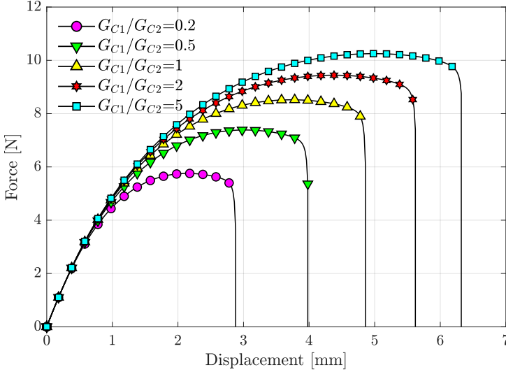
Figure 49: Reaction force-imposed displacement curves for the parametric study changing the critical energy release rate ratio with residual stress parameters \bar{\alpha}_c = 0.5 - \bar{\alpha}_d = 40 .
