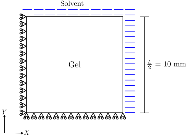
Figure 78: Configuration for the 2-D free swelling and thermal deswelling problem.
