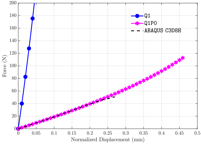
Figure 56: Reaction force-displacement curves for the benchmark problem run with Q1 and Q1P0 algorithms compared with ABAQUS C3D8H elements, respectively.
