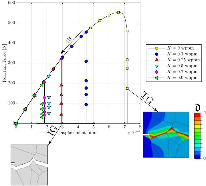
Figure 15: Predicted force versus displacement curves for the 10-grain SENT benchmark. The results are presented as a function of the environmental hydrogen concentration C_{env} , and images are embedded to showcase the different intergranular (IG) and transgranular (TG) cracking patterns observed.
