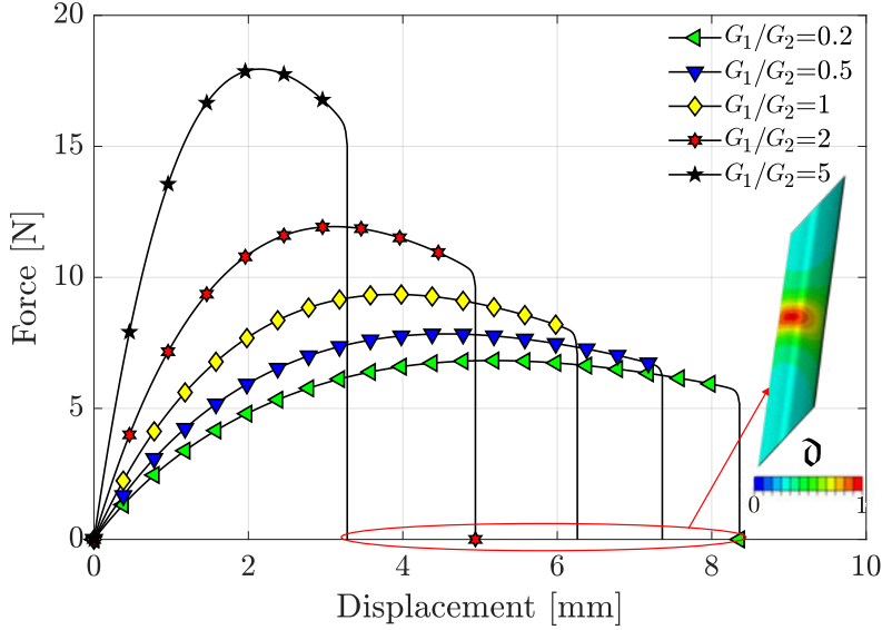
Figure 45: Reaction force-imposed displacement curves for the parametric study changing the shear modulus ratio without residual stress.
