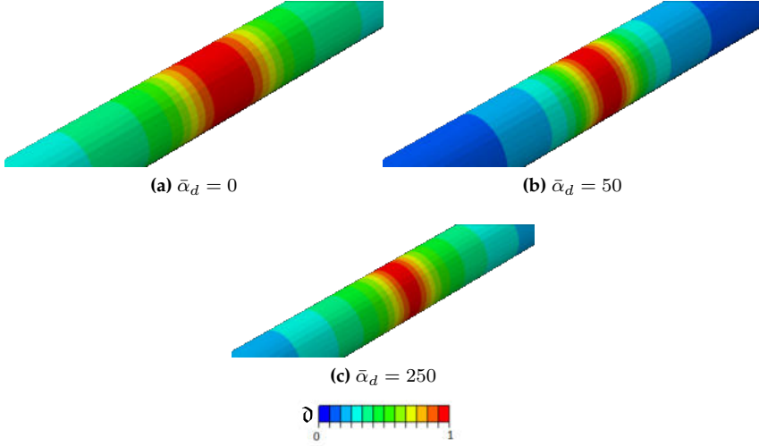
Figure 39: Phase field isocontour at the moment of failure for the residually stressed hollow cylinder with different values of \bar{\alpha}_d .
