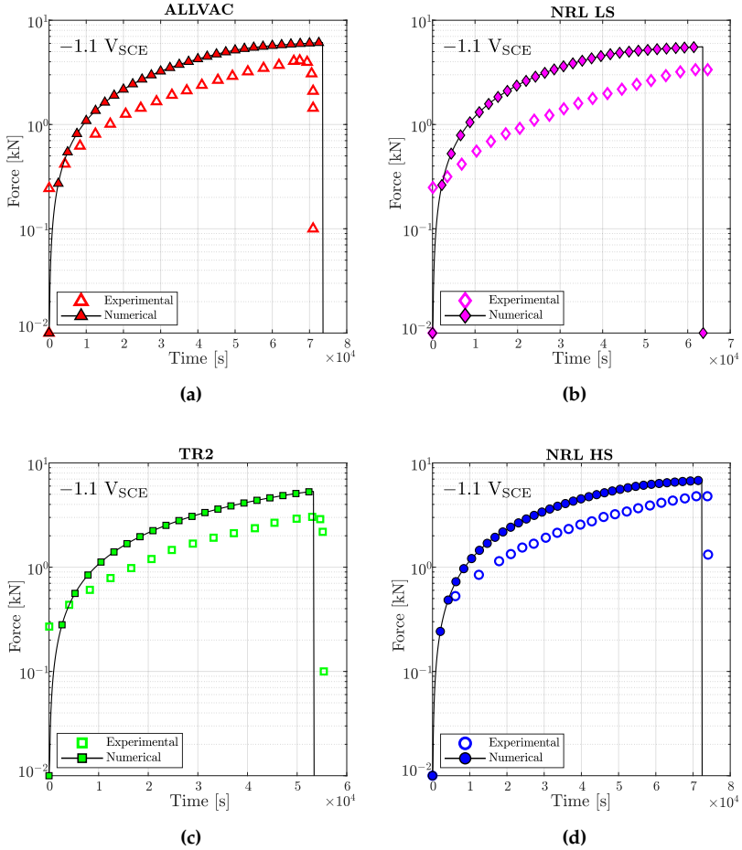
Figure 23: Virtual SSRT experiments on Monel K-500: numerical and experimental force versus time curves obtained under an applied potential of E_A = -1.1 V_{SCE} for each material lot; namely, (a) Allvac, (b) NRL LS, (c) TR2 and (d) NRL HS.
