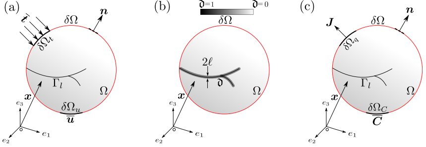
Figure 9: Schematic representation of the three-field boundary value problem: (a) displacement, (b) phase-field fracture, and (c) hydrogen diffusion.
