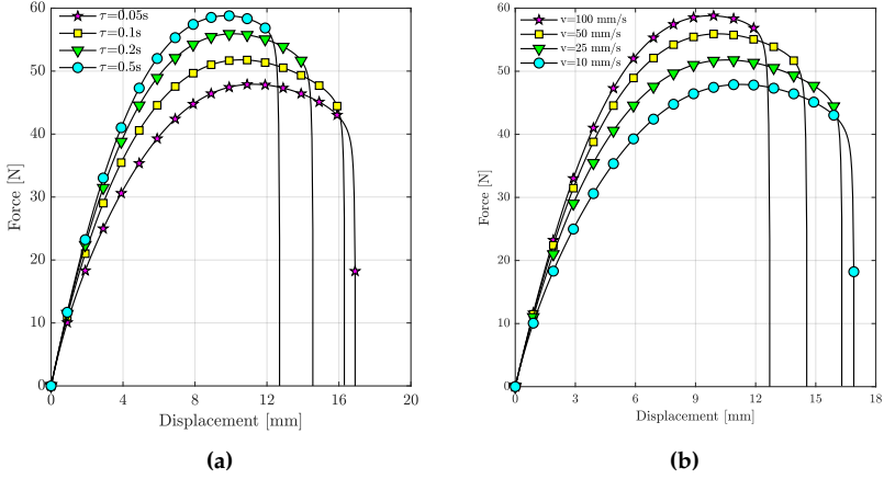
Figure 33: Load-displacement curves for cases with different (a) relaxation times and (b) displacement velocities for the non pre-stressed cylinders.
