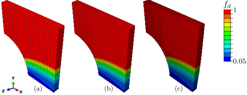
Figure 61: Isocontour plots for the damage function f_d comparing a (a) coarse, (b) medium-sized, and (c) fine discretisation of a plate with a hole with a fixed displacement of u_z = 8 mm. The obtained results are similar for Q1Q1 and Q1Q1E24 formulations.
