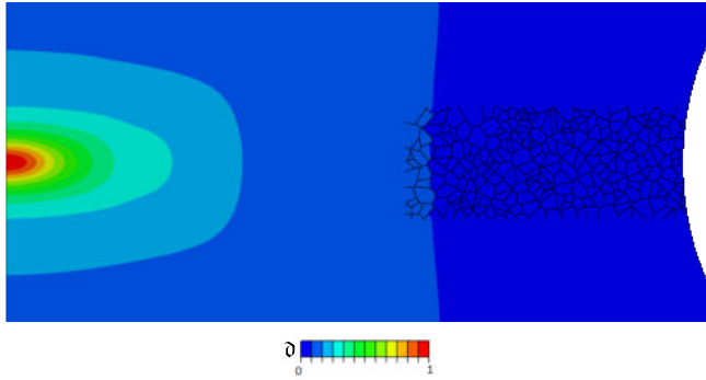
Figure 20: Virtual SSRT experiments on Monel K-500: phase field fracture contour at the time of crack initiation. In the absence of hydrogen, cracking takes place at the centre of the sample, in agreement with experimental observations.
