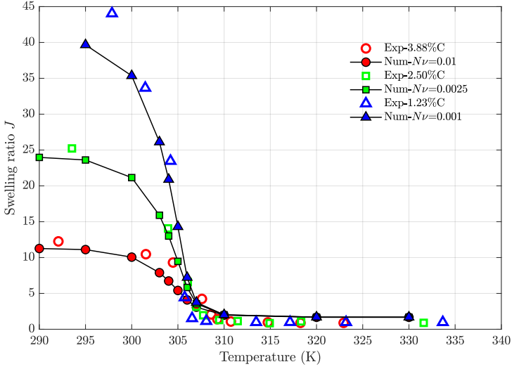
Figure 88: Volume of free-swelling hydrogel depending on temperature for different crosslinking densities. To adjust for the different experiments of [349], we have changed the parameter N\nu .
