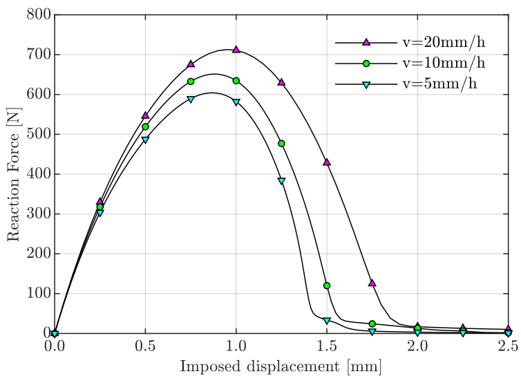
Figure 53: Load-displacement curves for tests of the single-notched square plate with different testing rates.
