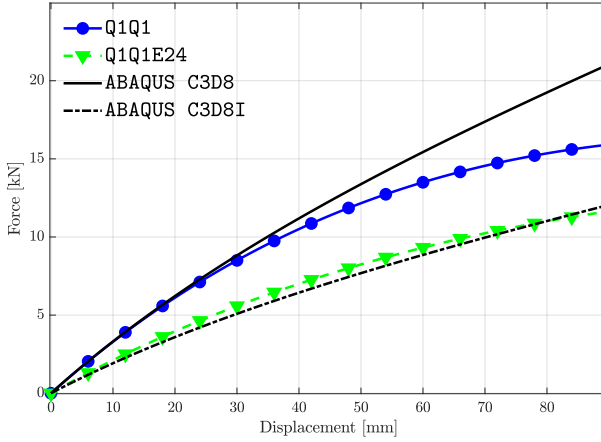
Figure 70: Load-displacement curves for the cylindrical shell test conducted for Q1Q1 and Q1Q1E24 formulations compared with the ABAQUS theoretical curves with (C3D8I) and without considering incompatible modes (C3D8). The employed saturation parameter has been \eta_d = 0.1 \text{ MPa}^{-1} .
