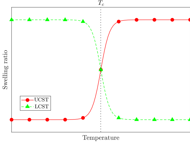
Figure 7: Symbolic graphic representation on the evolution against temperature for UCST and LCST hydrogels.
