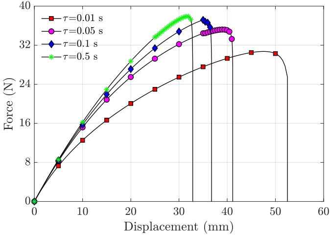
Figure 31: Load-displacement curves for tests with v = 500 mm/s and different relaxation times on the double-notched plane strain specimens.
