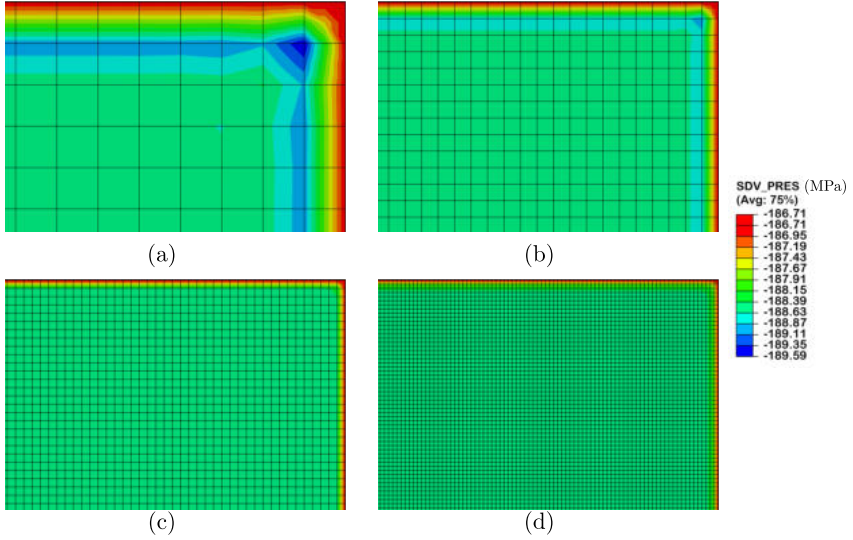
Figure 83: First increment of unloading pressure ramps conducted for discretizations with element sizes: (a) h = 0.15 , (b) h = 0.1 , (c) h = 0.05 and (d) h = 0.025 mm with a time step of \Delta t = 0.15 s. It is observed how by increasing discretization, the variation of the pressure becomes smooth.
