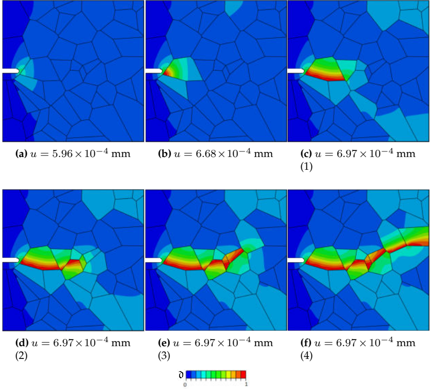
Figure 16: Crack evolution resulting in transgranular fracture for the 50-grain benchmark sample with C = 0 wppm sorted by displacement. Plotted is the phase-field parameter.
