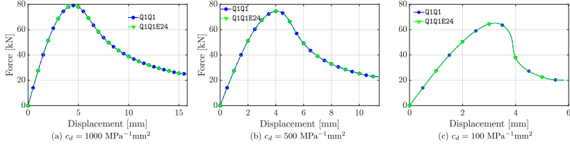
Figure 62: Reaction force-displacement curves for the compressible plate with a hole problem comparing standard CDM (Q1Q1) and CDM + EAS (Q1Q1E24) formulations varying c_d .
