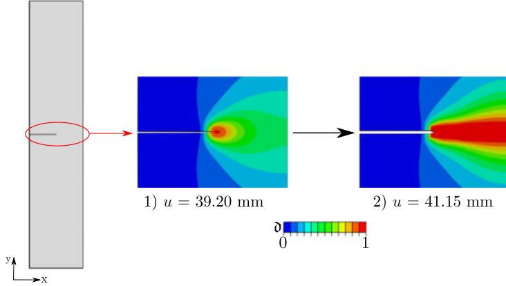
Figure 32: Zoom in the notched area during: Mode I (1) crack initiation and (2) propagation for the case with parameters v = 500\text{mm/s} and \tau = 0.1 s. Plotted is the phase field parameter isocontour with the legend case, where blue and red denote intact and broken states, respectively.
