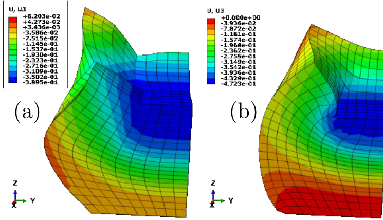
Figure 55: Isometric view from the deformed of the benchmark problem run with (a) Q1 and (b) Q1P0 algorithms, respectively.
