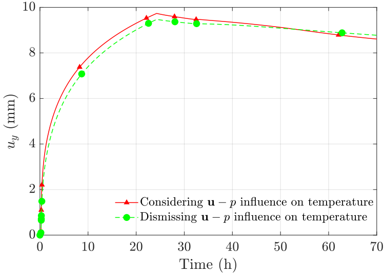
Figure 86: Time evolution of the vertical displacement in the top right node for the swelling-deswelling test with (red, continuous line) and without (green, dashed line) considering the fluid flow and elastic stretching influence on the temperature.
