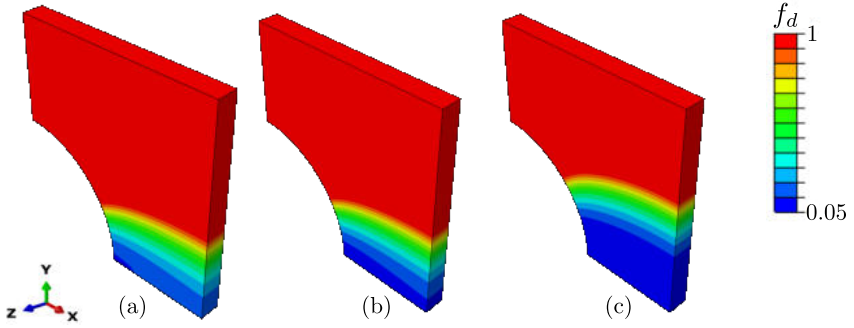
Figure 60: Isocontour plots for the damage function f_d of a plate with a hole plotting the crack pattern for several displacements: (a) u_z = 7.32 mm, (b) u_z = 8.42 mm and (c) u_z = 19.10 mm. Employed non-local damage parameters encompass: \eta_d = 1 \text{ MPa}^{-1} , \kappa_d = 1 \text{ MPa} and c_d = 500 \text{ MPa}^{-1}\text{mm}^2
