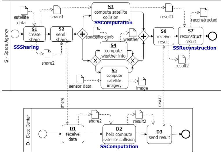
Figure 11: PE-BPMN model enhanced with data objects and secret sharing.
