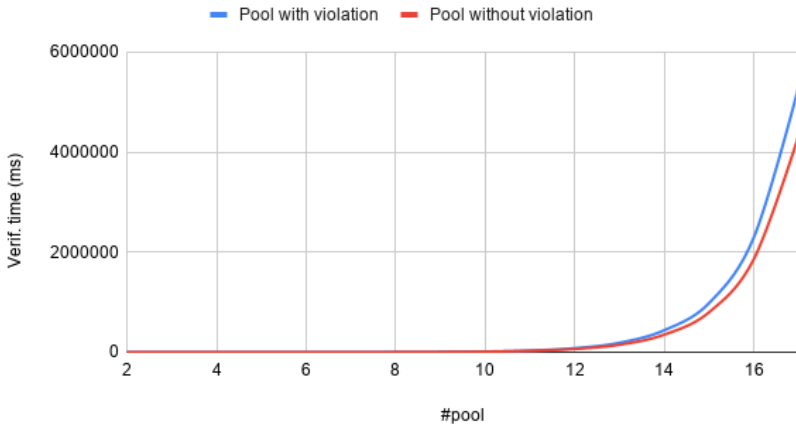
Figure 21: Chart showing how the verification time for PE-BPMN models in table 7 grows depending on the number of pools being in parallel.
