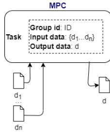
Figure 10: Multiparty computation.
