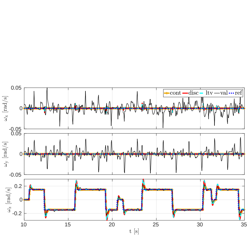
Figure 50: Body angular velocity from the yaw validation results. Yellow, red, and cyan lines represent the continuous-time nonlinear, discrete-time nonlinear, and discrete-time LTV models, respectively. Black and dotted blue lines correspond to the validation data and references to the PD controller
