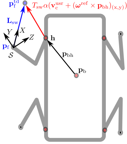
Figure 27: Representation of the robocentric stepping strategy and of the Swing Frame, located at the lift-off point. The red arrow shows the distance between the touchdown point p_f^{td} and the hip h . The blue vector L_{sw} connects lift-off and touchdown point.
