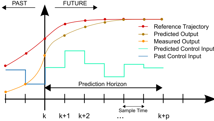
Figure 15: Illustration of the RHP utilized in the MPC scheme (Source: Behrendt (2009)).
