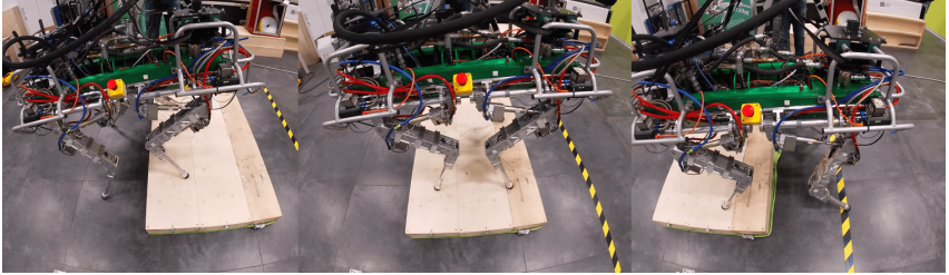
Figure 36: IIT's quadruped robot HyQ traversing a static pallet with the mobility enhanced real-time NMPC.
