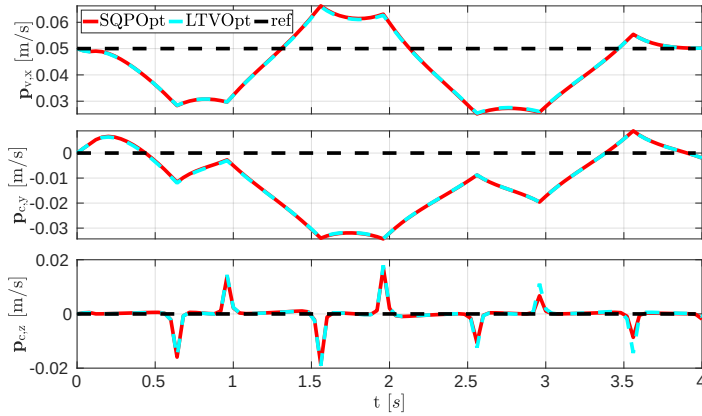
Figure 18: CoM velocity plots from LTVOpt and SQPOpt results. Red line is the output of SQPOpt, dashed cyan line is the result of LTVOpt and black dashed line is CoM reference velocity.
