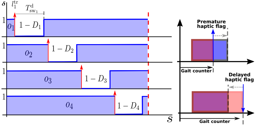
Figure 26: Gait schedule for a walk. Offsets \mathbf{o} = [0.05, 0.3, 0.55, 0.8] , duty-factors \mathbf{D}_f = [0.85, 0.85, 0.85, 0.85] . The red arrows represent the trigger l_i^{tr} for a swing leg i . Right part shows the fast-forwarding (top) or re-winding (bottom) of the gait counter to recover synchronization between actual (haptic) and planned touchdown.
