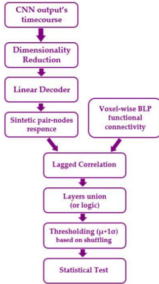
Figure 2.1 Preprocessing pipeline The description of preprocessing steps of CNN output and BLP FC
