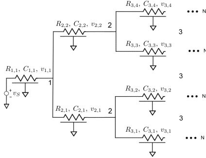
Figure 3: H-tree network adapted from [133].
