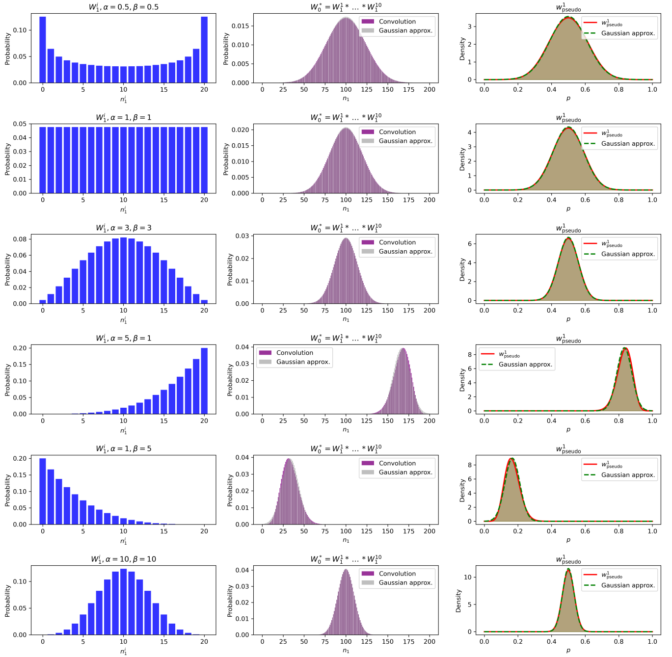
FIG. S5. The first column shows the discrete distribution of each component of the alternative sufficient statistics, here denoted simply by W_1^i , induced by independent identical beta priors on the alternative, for different prior parameters. The GRO-optimal microcanonical prior on the null W_0^* (second column) for the 2 \times k test is obtained by convolving these discrete distributions k times. The pseudo prior density w_{pseudo}^1 (third column) is instead obtained by directly convolving k times the corresponding beta priors. Both W_0^* and w_{pseudo}^1 are shown together with their Gaussian approximations (discrete for W_0^* and continuous for w_{pseudo}^1 ). In this example, k = 10 .
