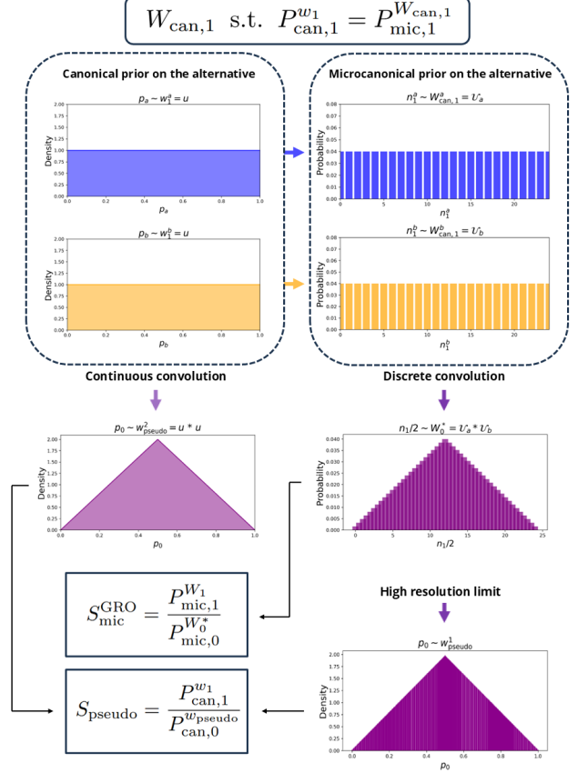
FIG. 4. Procedures to compute the microcanonical approximation S_{\text{mic}}^{\text{GRO}} and the pseudo approximation S_{\text{pseudo}} for testing between two binary data streams, under uniform priors (as in Examples A, B, and C). Starting from two independent continuous uniform priors on the alternative (top left), we construct discrete microcanonical priors (top right) satisfying P_{\text{can},1}^{w_1} = P_{\text{mic},1}^{W_{\text{can},1}^*} . The optimal discrete prior W_0^* , used in S_{\text{mic}}^{\text{GRO}} , is obtained by convolving the alternative priors. The continuous prior w_{\text{pseudo},0} for S_{\text{pseudo}} is derived either from W_0^* through a high resolution limit ( w_{\text{pseudo},0}^1 ), or by directly convolving the original continuous priors ( w_{\text{pseudo},0}^2 ).
