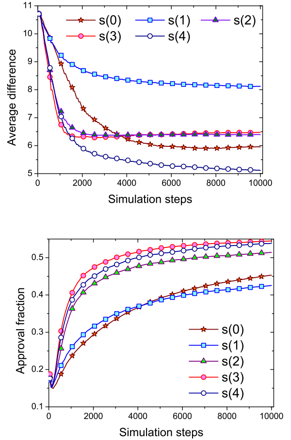
Fig. 2. Evolution of average differences (upper panel) and approval fraction (lower panel) in the adaptive system ruled by different definitions of the similarity. Refer to the next section for the definition of s^{(4)} .
